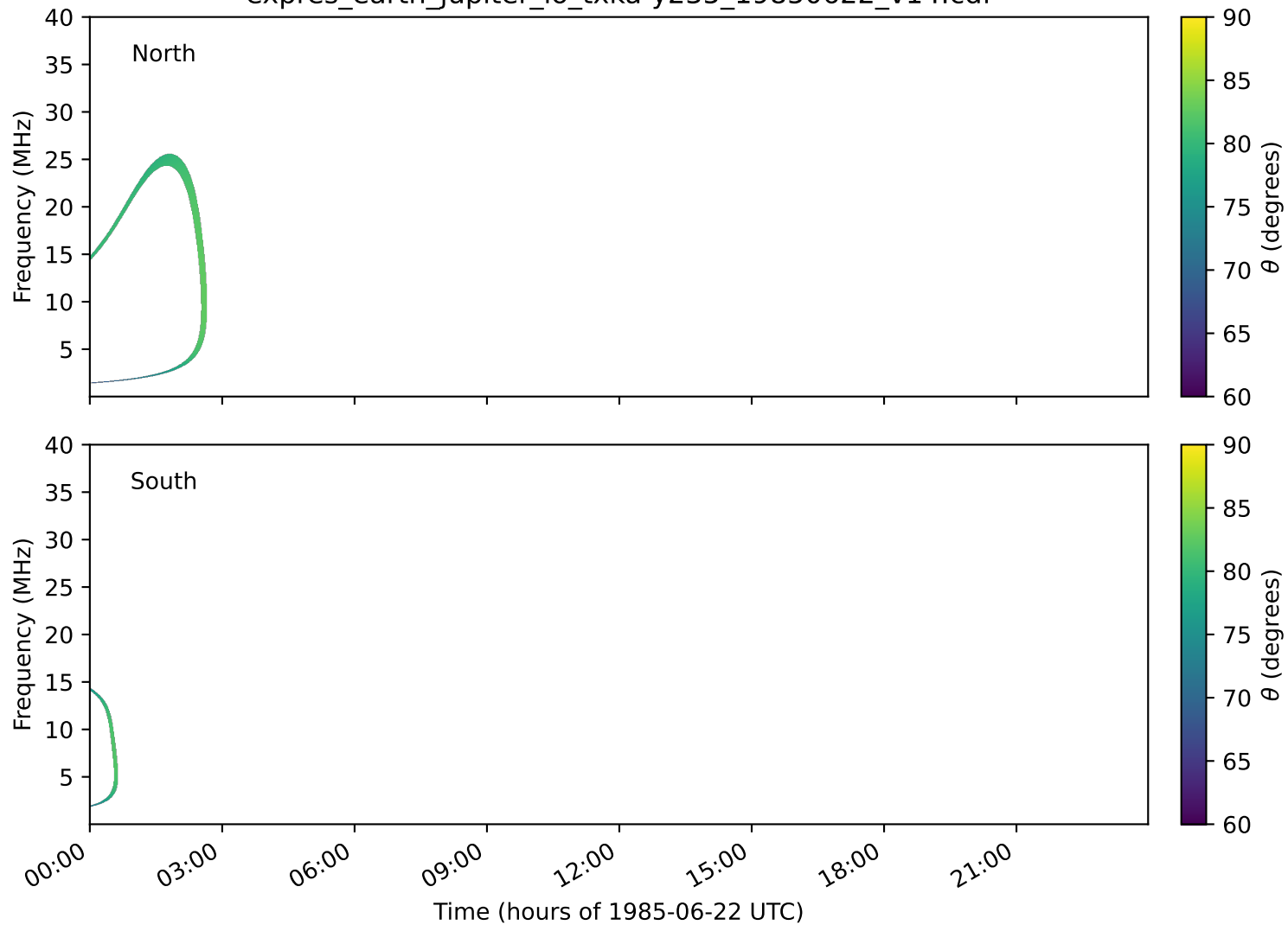
expres_earth_jupiter_io_txka-y235_19850622_v14.cdf
