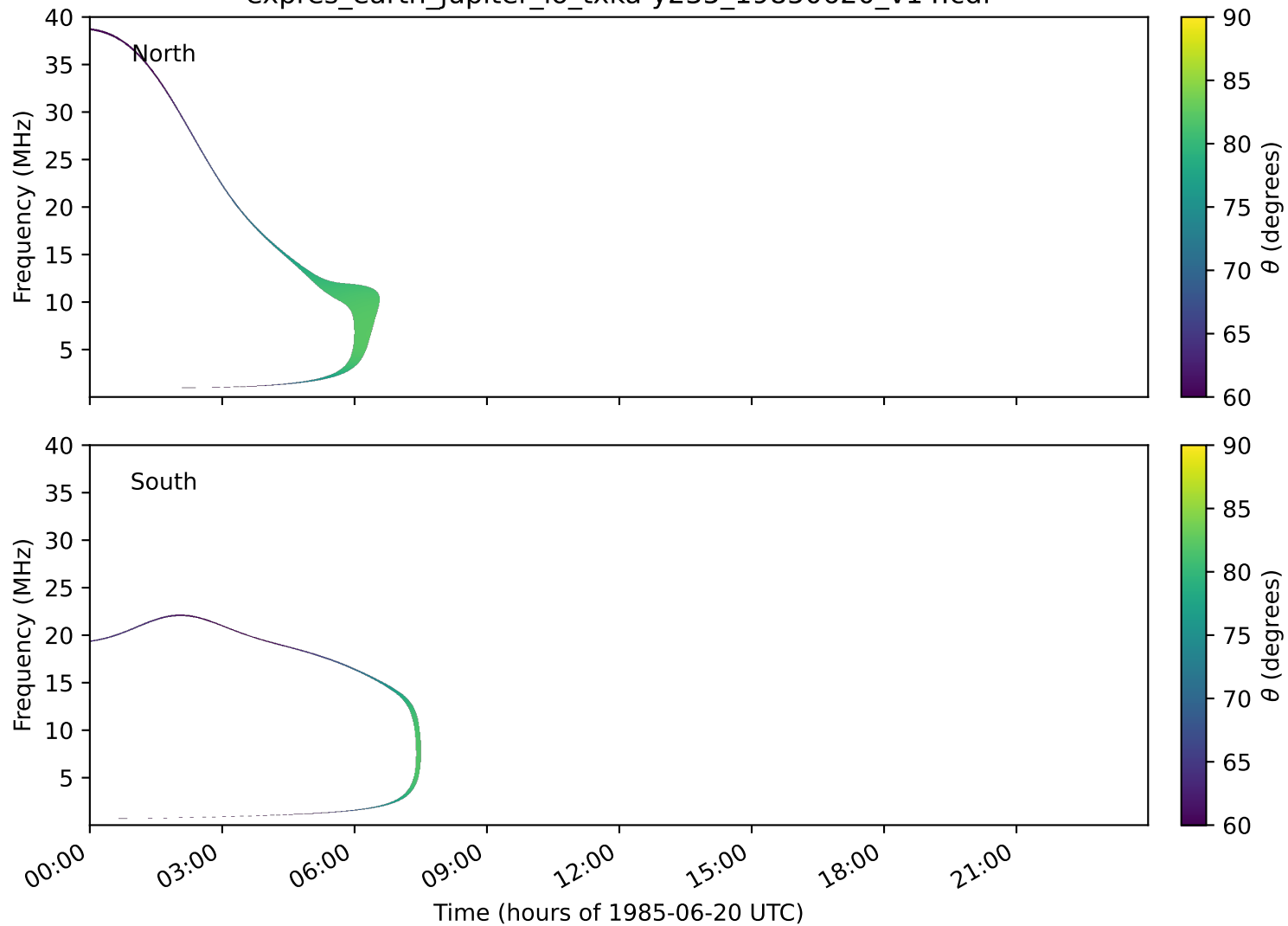
expres_earth_jupiter_io_txka-y235_19850620_v14.cdf
