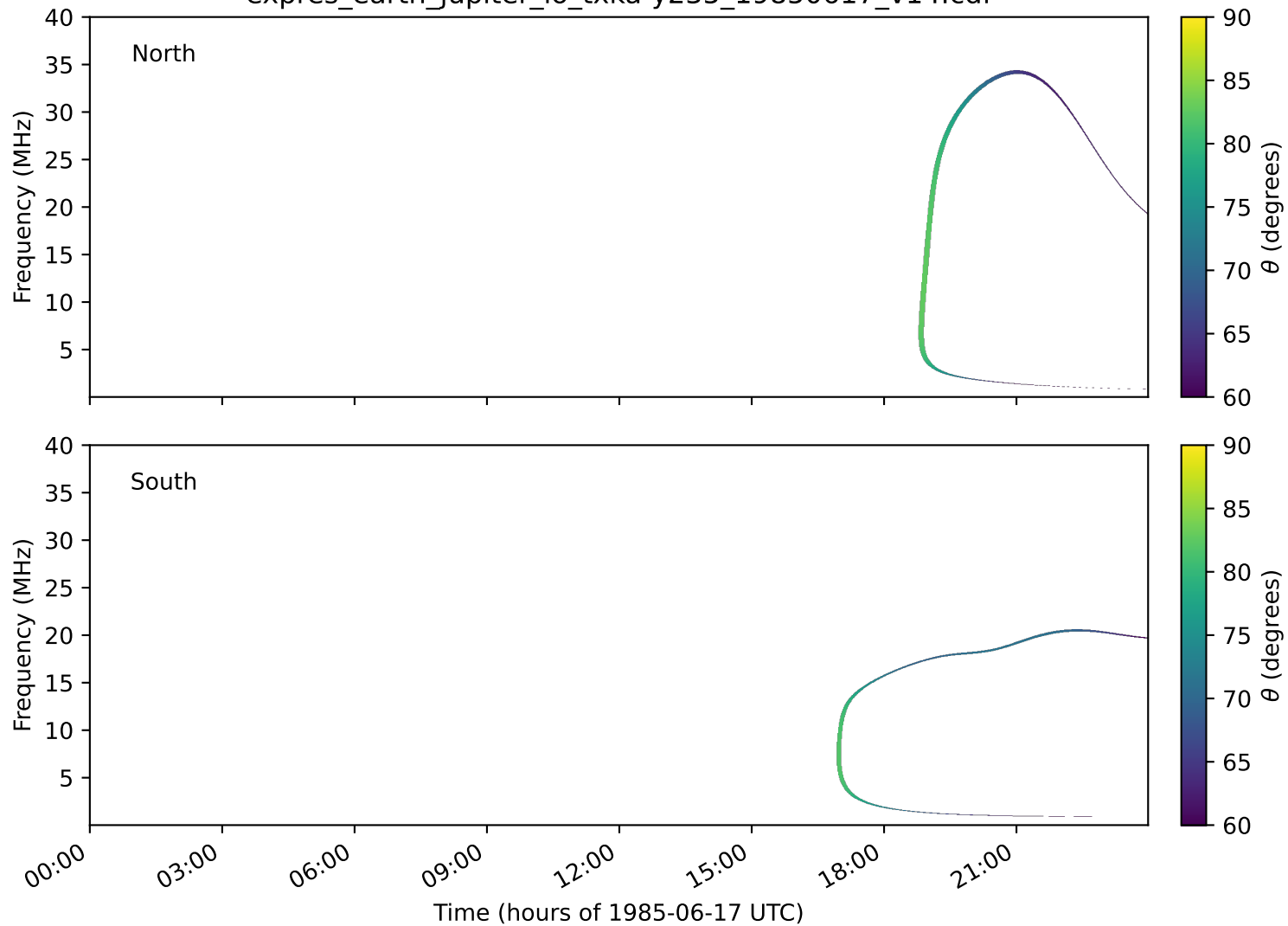
expres_earth_jupiter_io_txka-y235_19850617_v14.cdf
