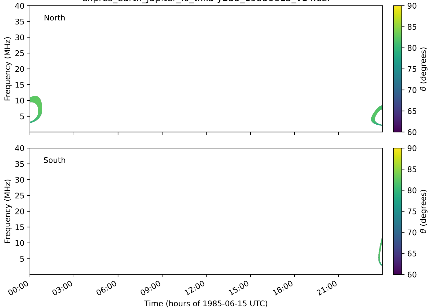
expres_earth_jupiter_io_txka-y235_19850615_v14.cdf
