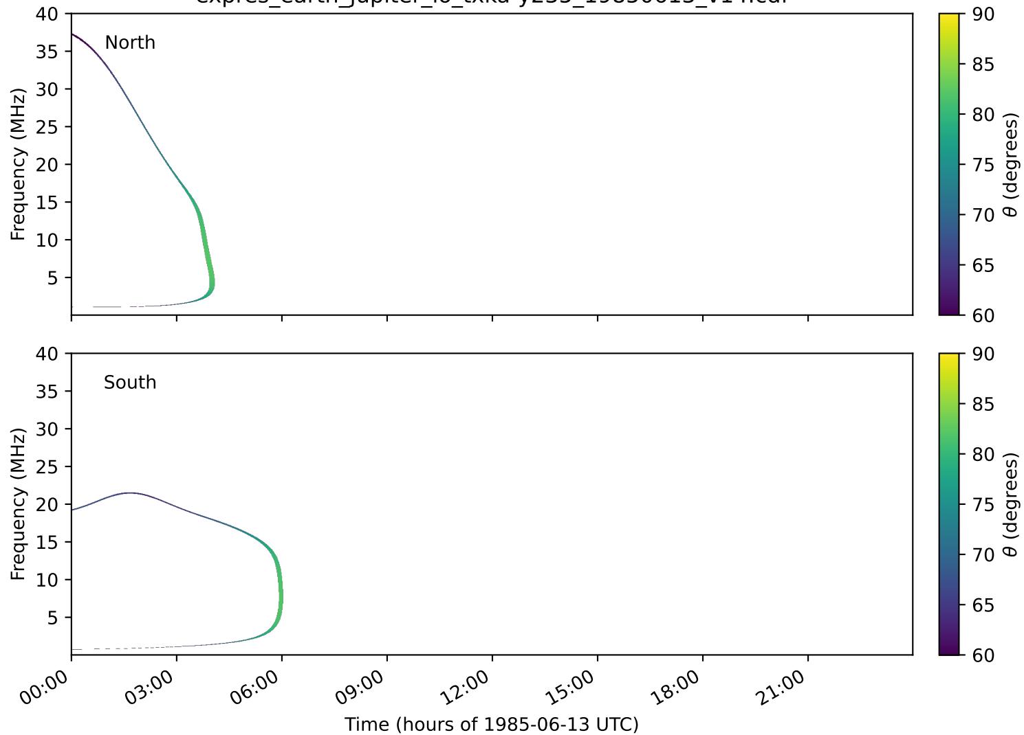
expres_earth_jupiter_io_txka-y235_19850613_v14.cdf
