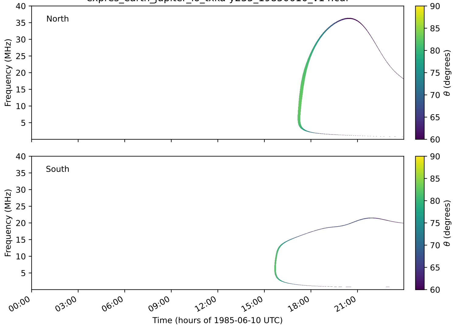
expres_earth_jupiter_io_txka-y235_19850610_v14.cdf
