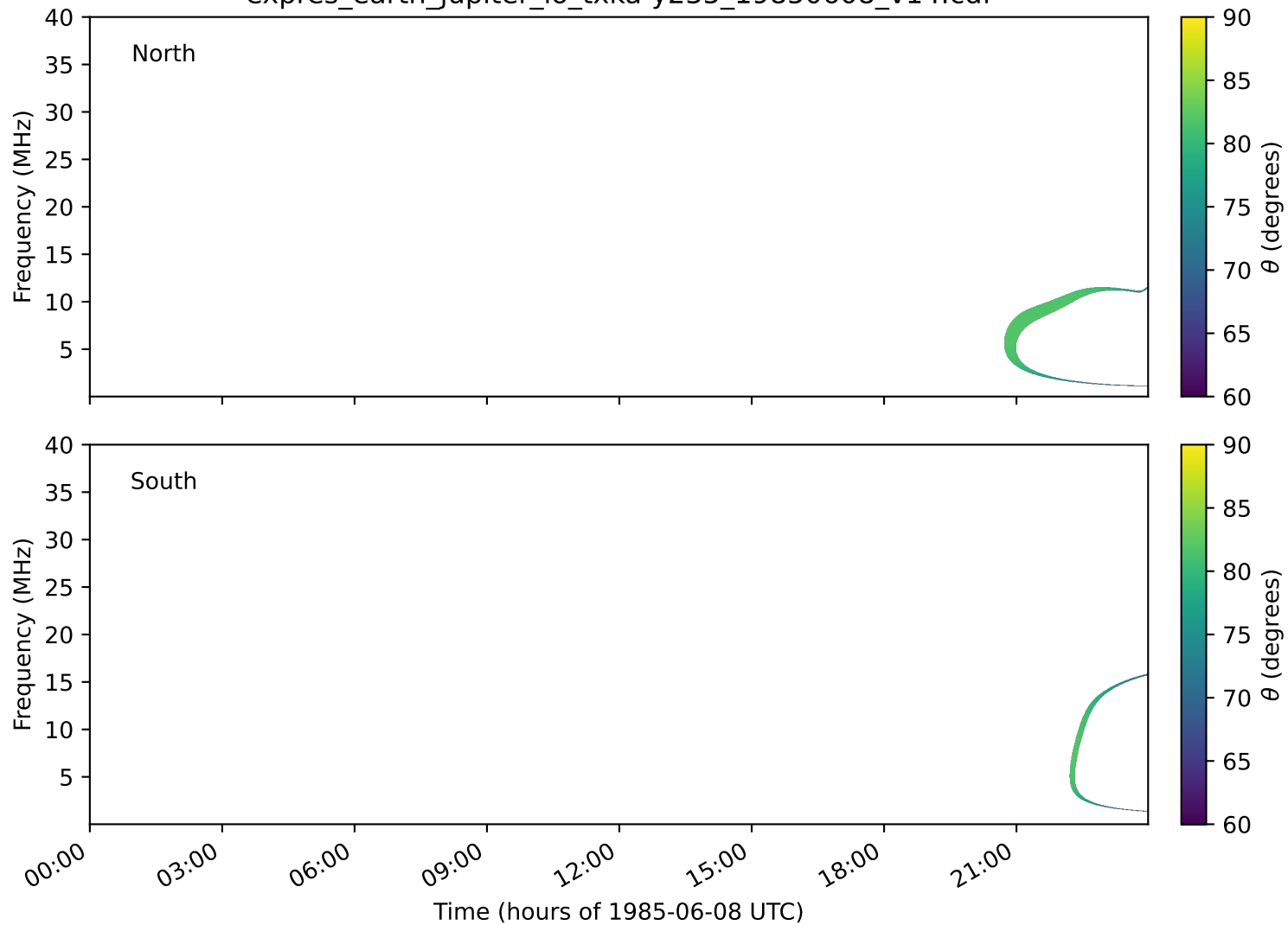
expres_earth_jupiter_io_txka-y235_19850608_v14.cdf
