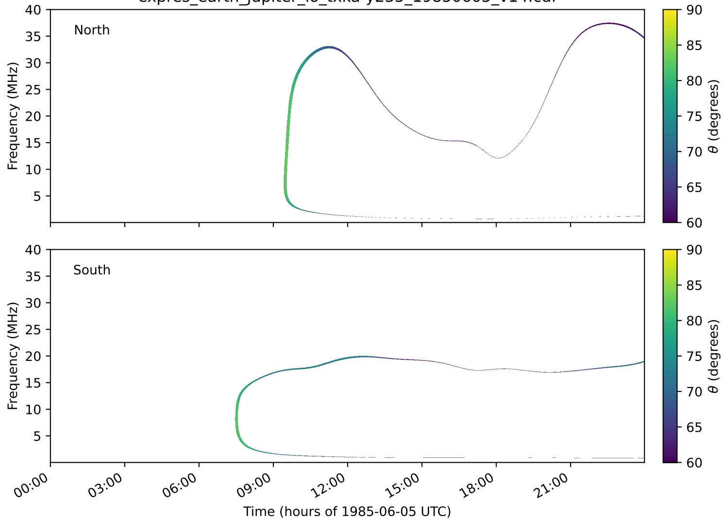
expres_earth_jupiter_io_txka-y235_19850605_v14.cdf
