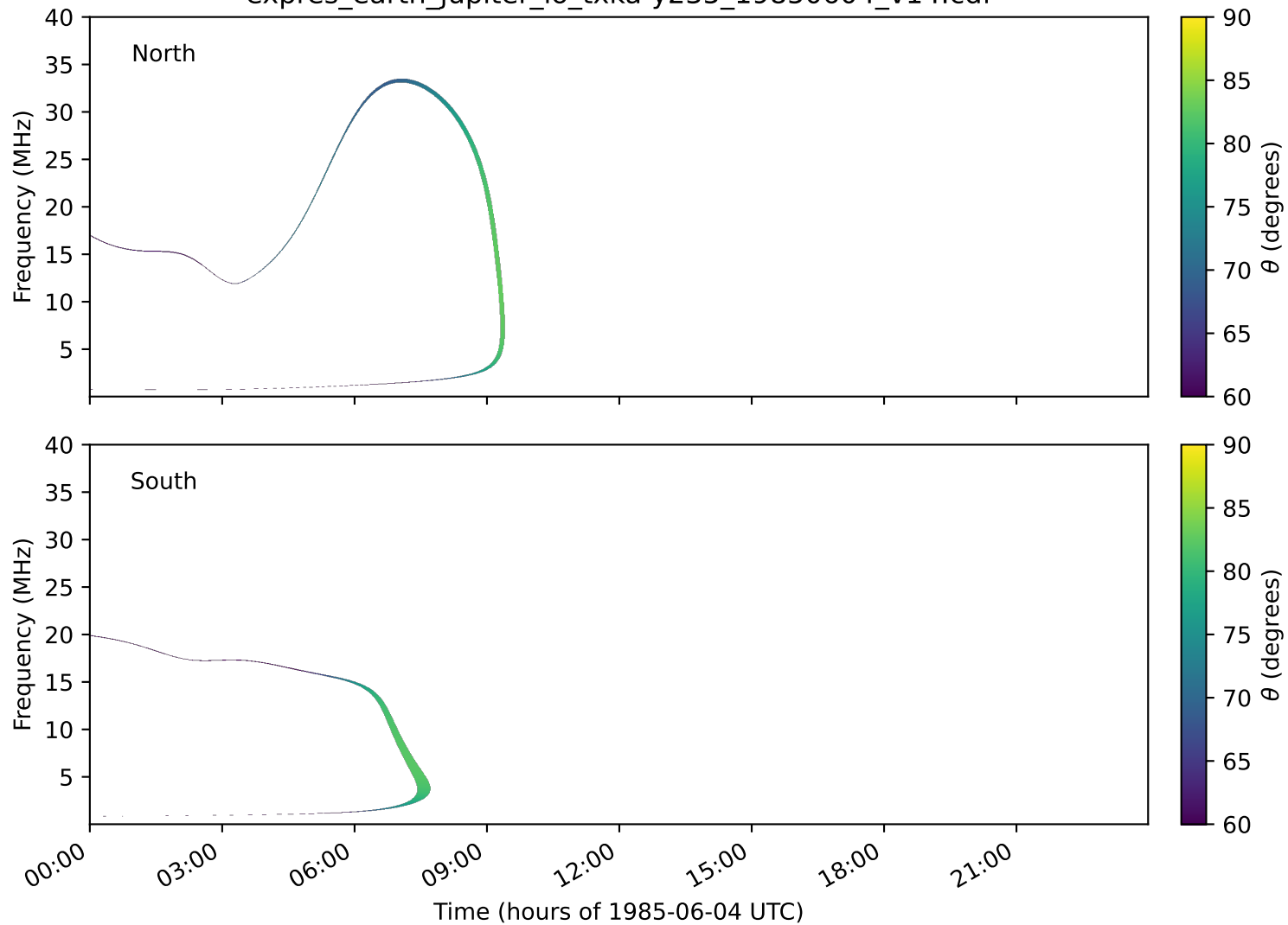
expres_earth_jupiter_io_txka-y235_19850604_v14.cdf
