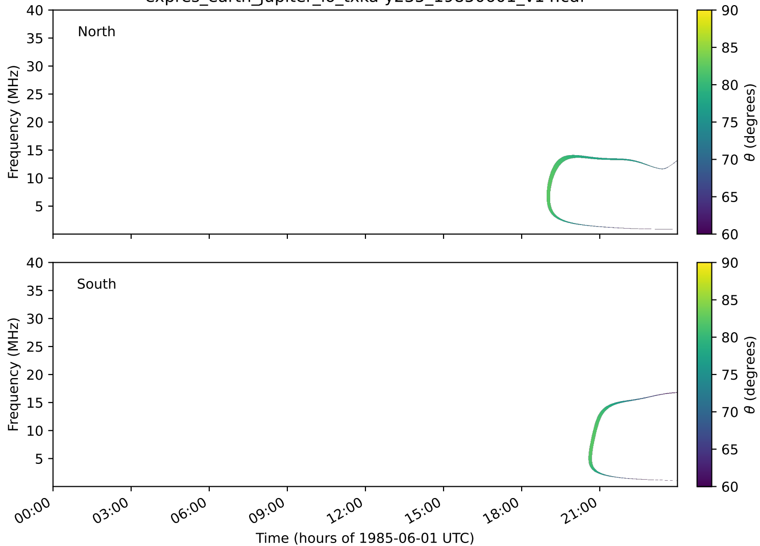
expres_earth_jupiter_io_txka-y235_19850601_v14.cdf
