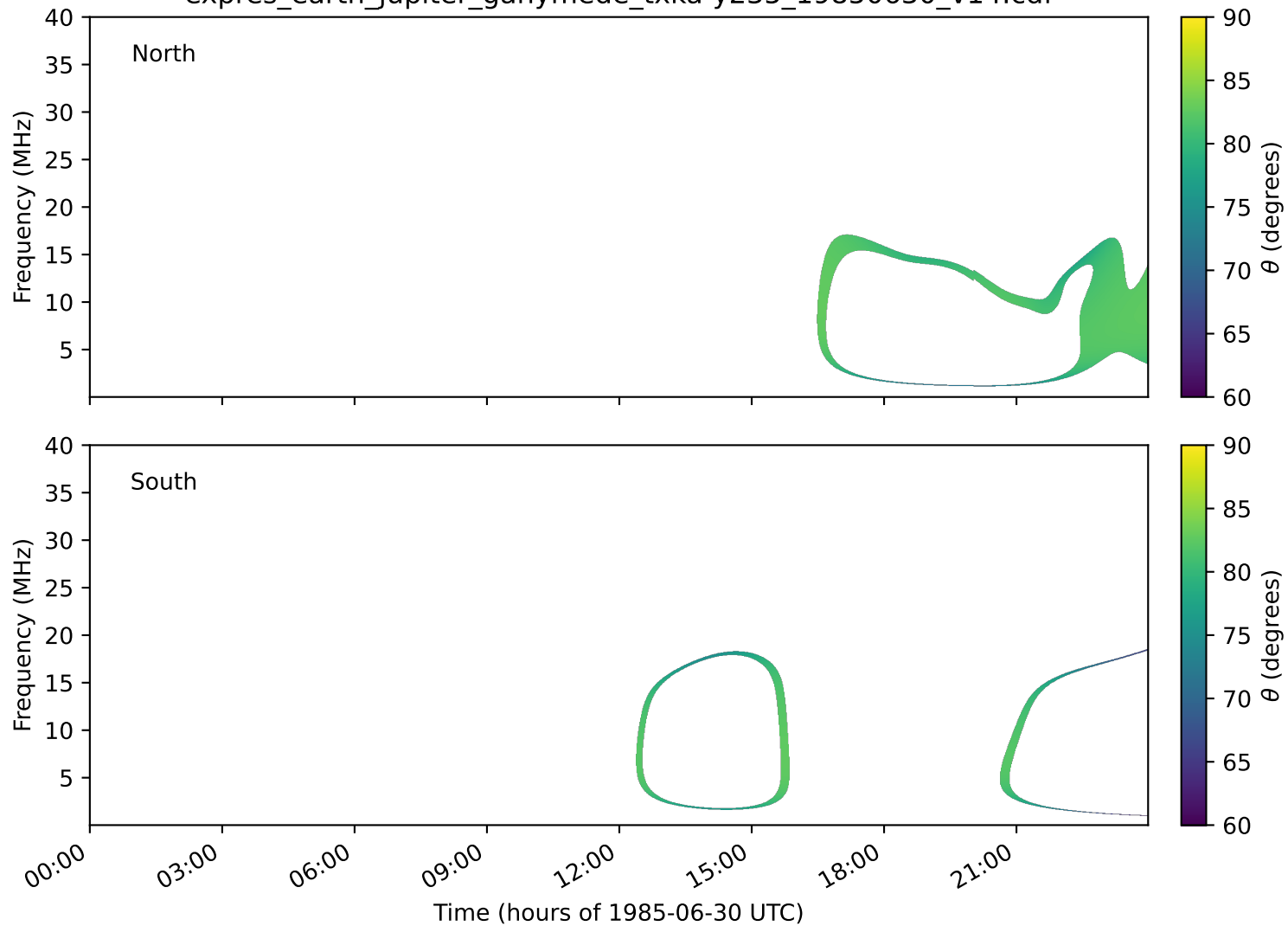
expres_earth_jupiter_ganymede_txka-y235_19850630_v14.cdf
