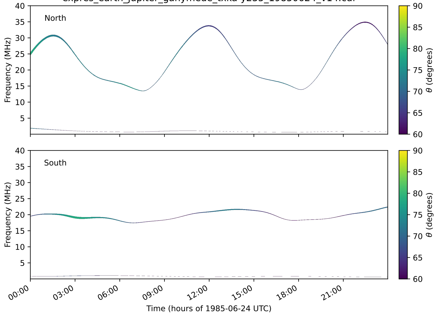
expres_earth_jupiter_ganymede_txka-y235_19850624_v14.cdf
