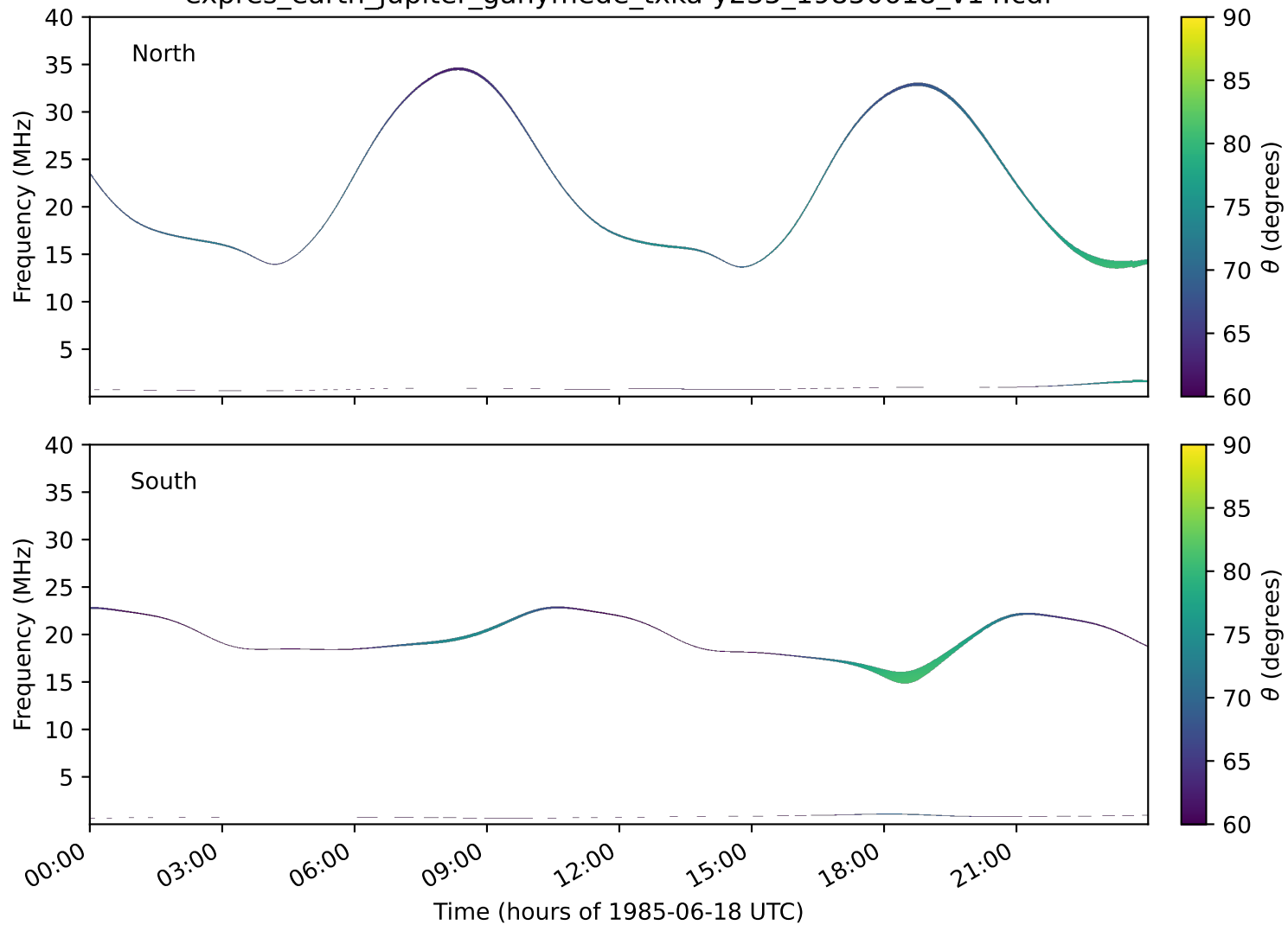
expres_earth_jupiter_ganymede_txka-y235_19850618_v14.cdf
