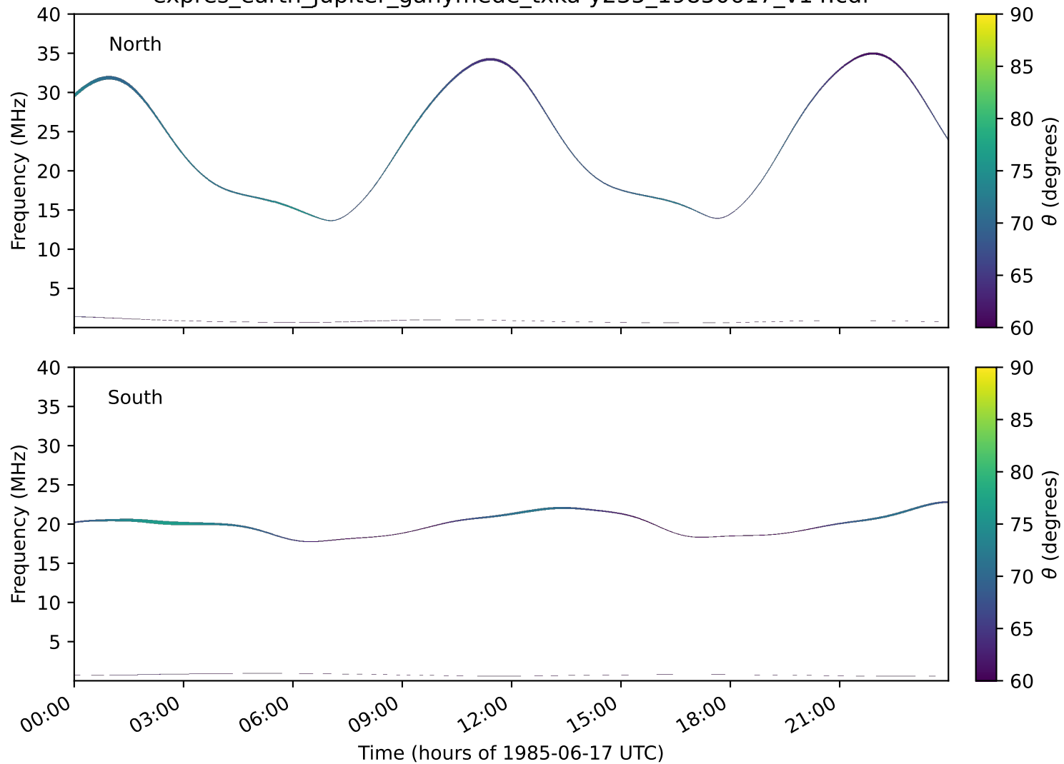
expres_earth_jupiter_ganymede_txka-y235_19850617_v14.cdf
