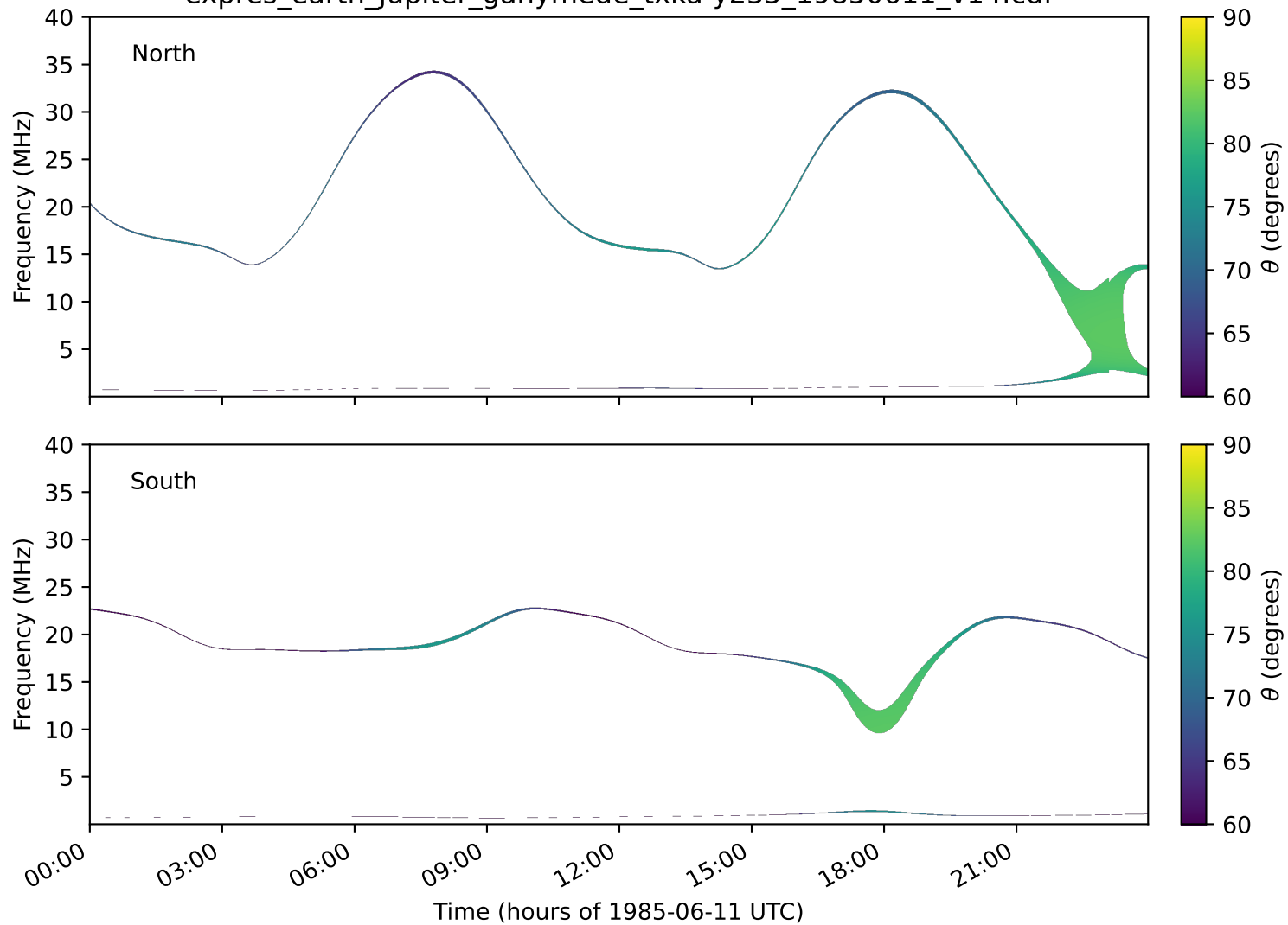
expres_earth_jupiter_ganymede_txka-y235_19850611_v14.cdf
