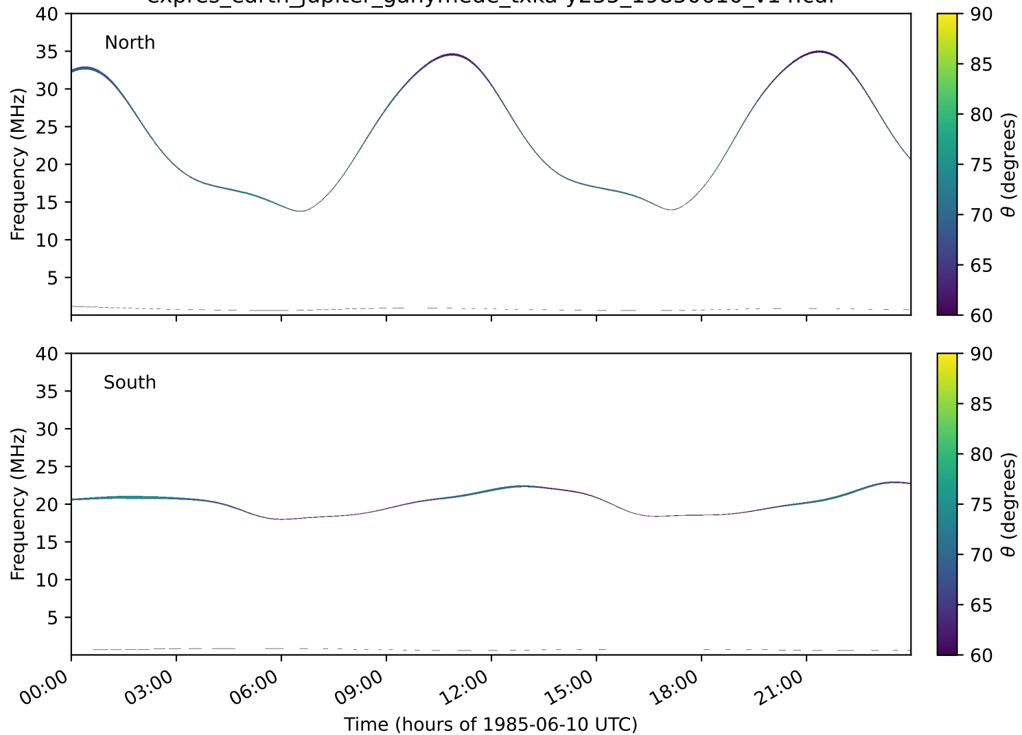
expres_earth_jupiter_ganymede_txka-y235_19850610_v14.cdf
