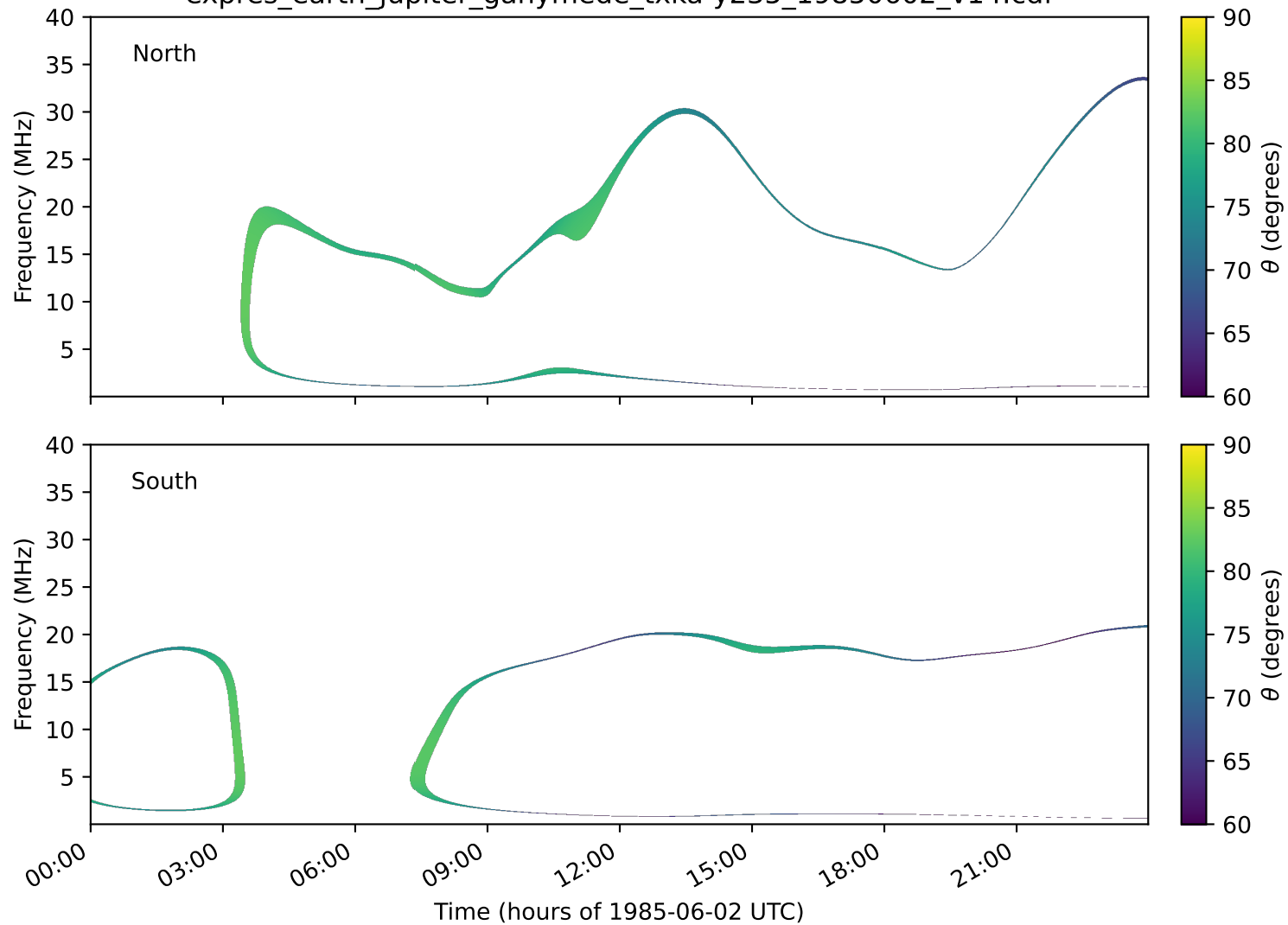
expres_earth_jupiter_ganymede_txka-y235_19850602_v14.cdf
