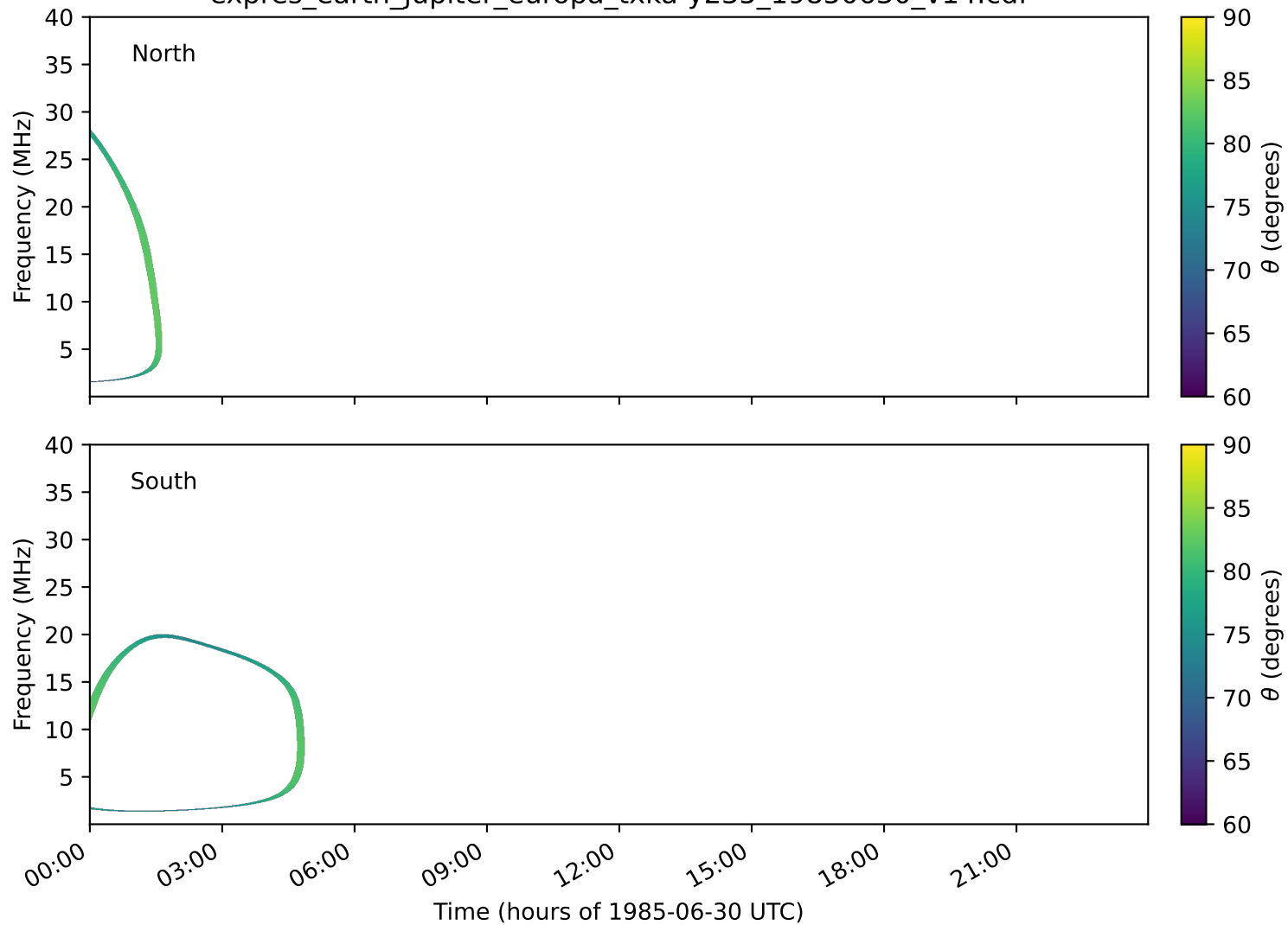
expres_earth_jupiter_europa_txka-y235_19850630_v14.cdf
