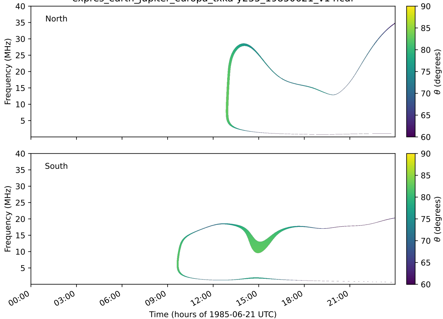
expres_earth_jupiter_europa_txka-y235_19850621_v14.cdf
