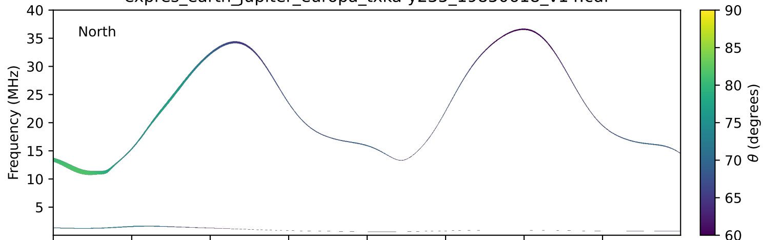
expres_earth_jupiter_europa_txka-y235_19850618_v14.cdf
