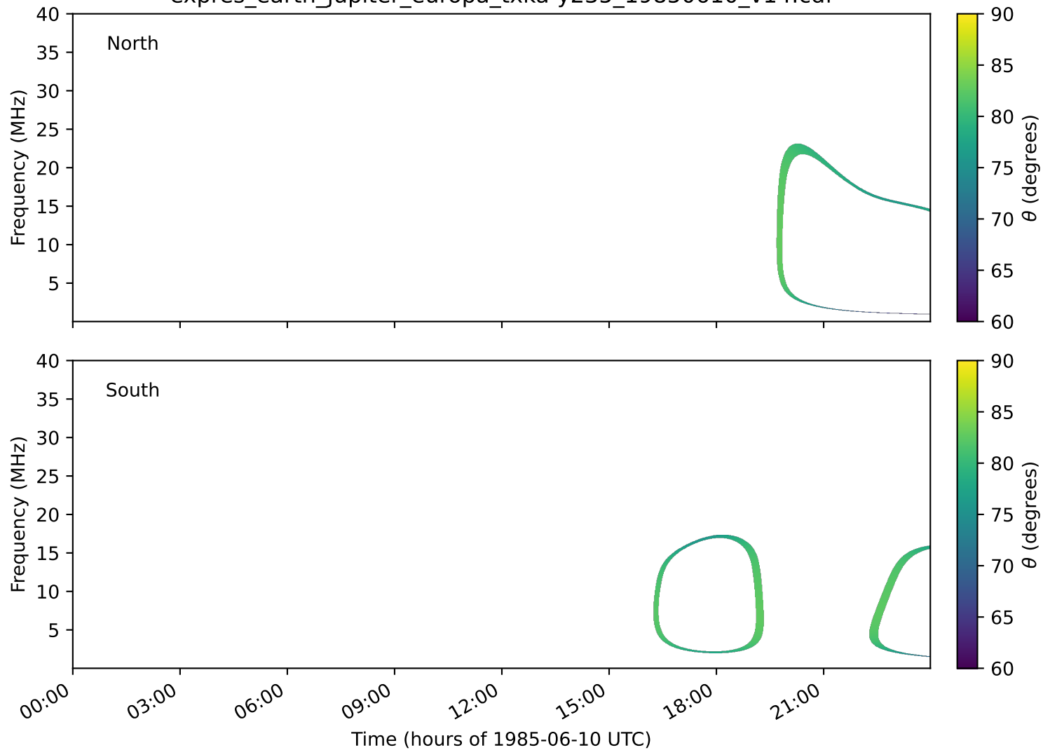
expres_earth_jupiter_europa_txka-y235_19850610_v14.cdf
