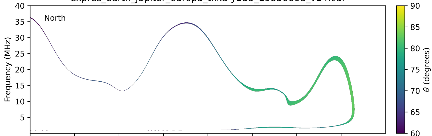
expres_earth_jupiter_europa_txka-y235_19850608_v14.cdf
