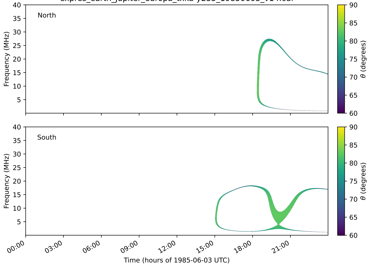
expres_earth_jupiter_europa_txka-y235_19850603_v14.cdf
