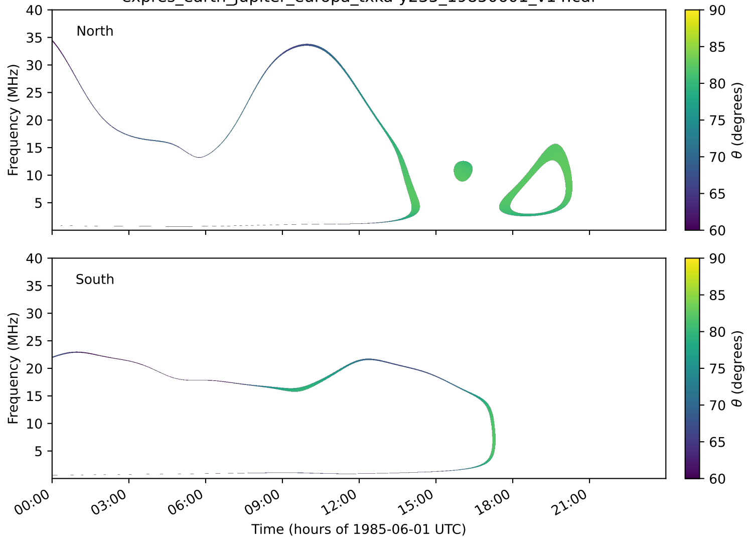
expres_earth_jupiter_europa_txka-y235_19850601_v14.cdf
