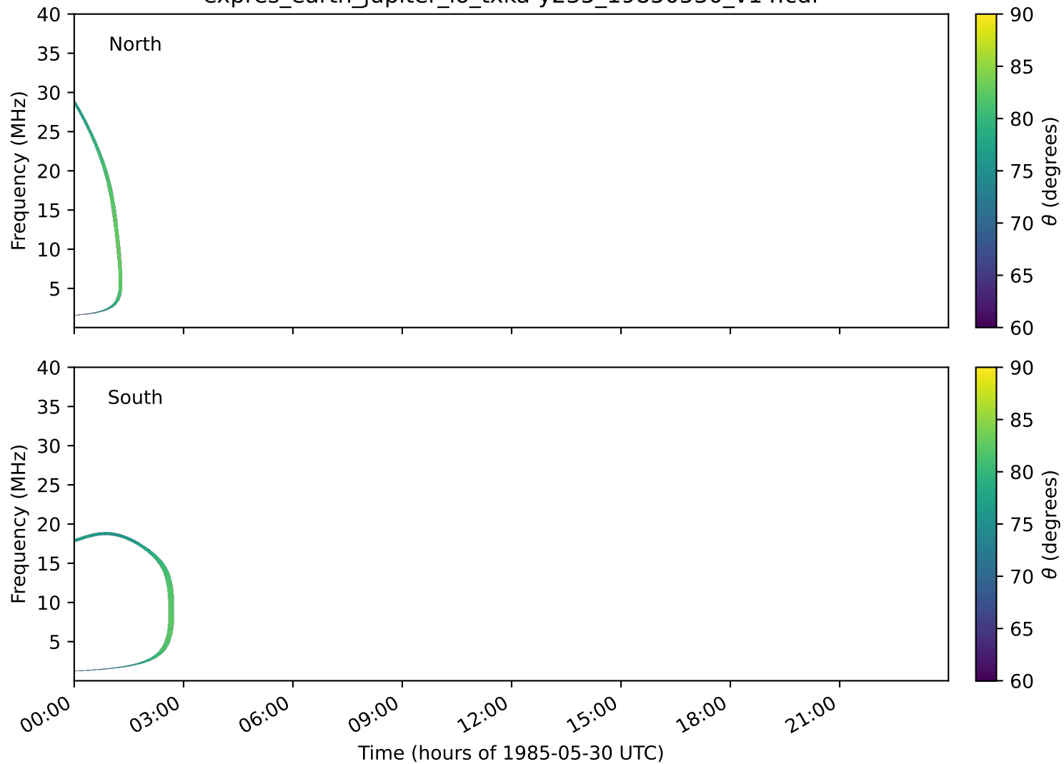
expres_earth_jupiter_io_txka-y235_19850530_v14.cdf
