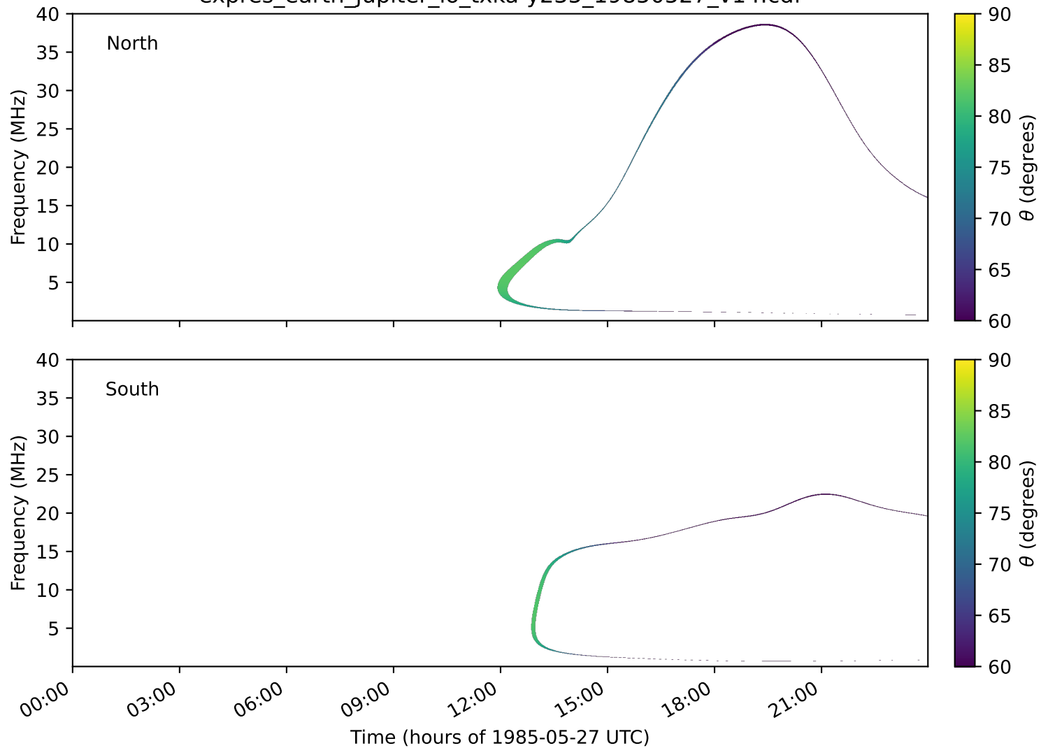
expres_earth_jupiter_io_txka-y235_19850527_v14.cdf
