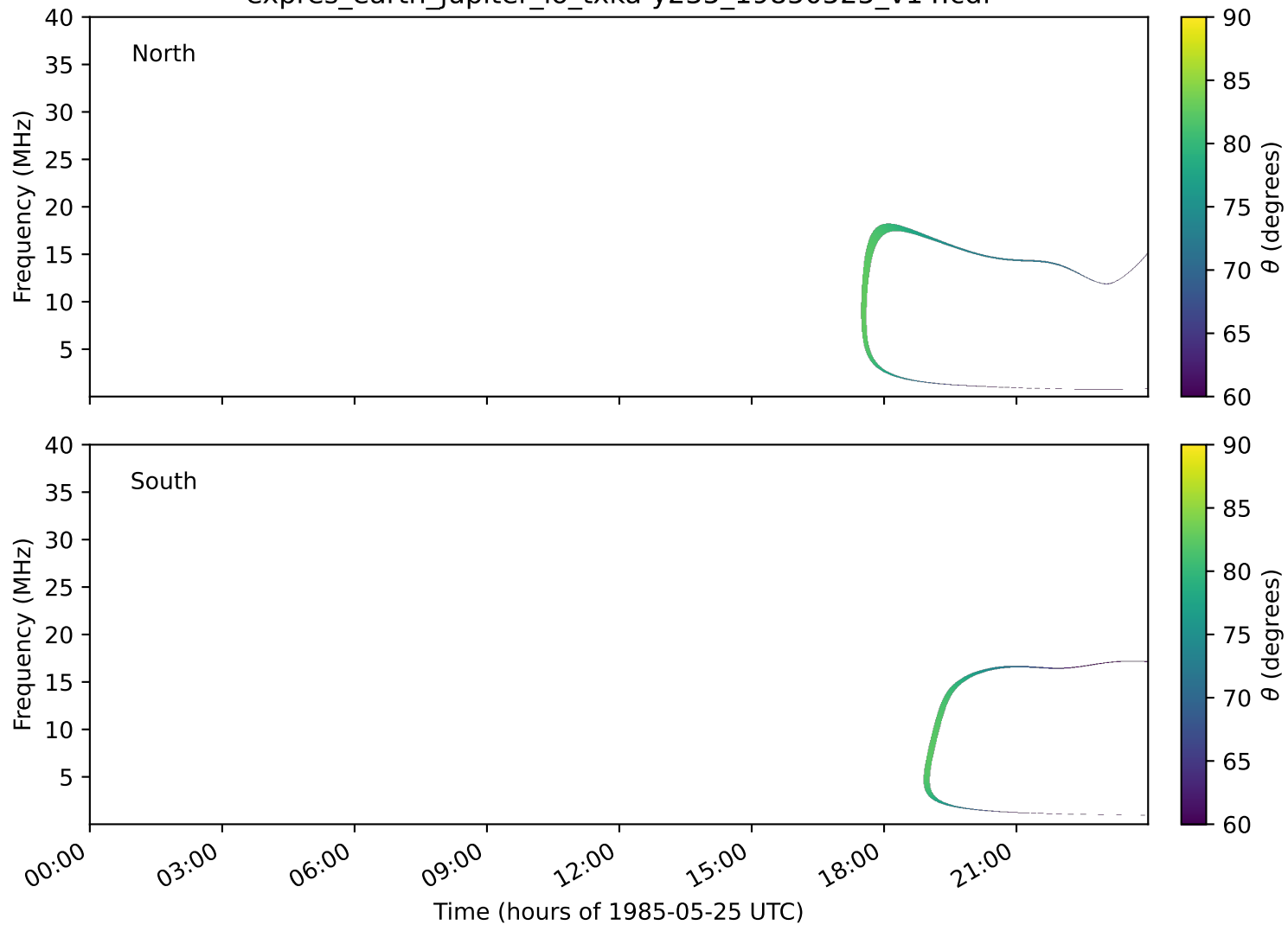
expres_earth_jupiter_io_txka-y235_19850525_v14.cdf
