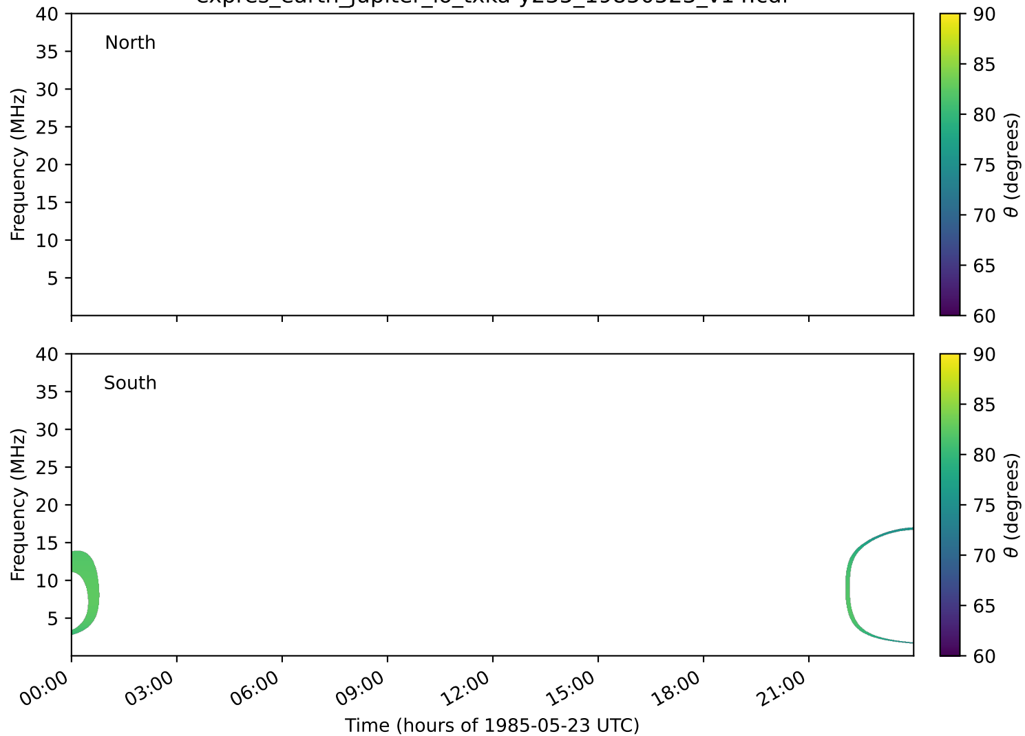
expres_earth_jupiter_io_txka-y235_19850523_v14.cdf
