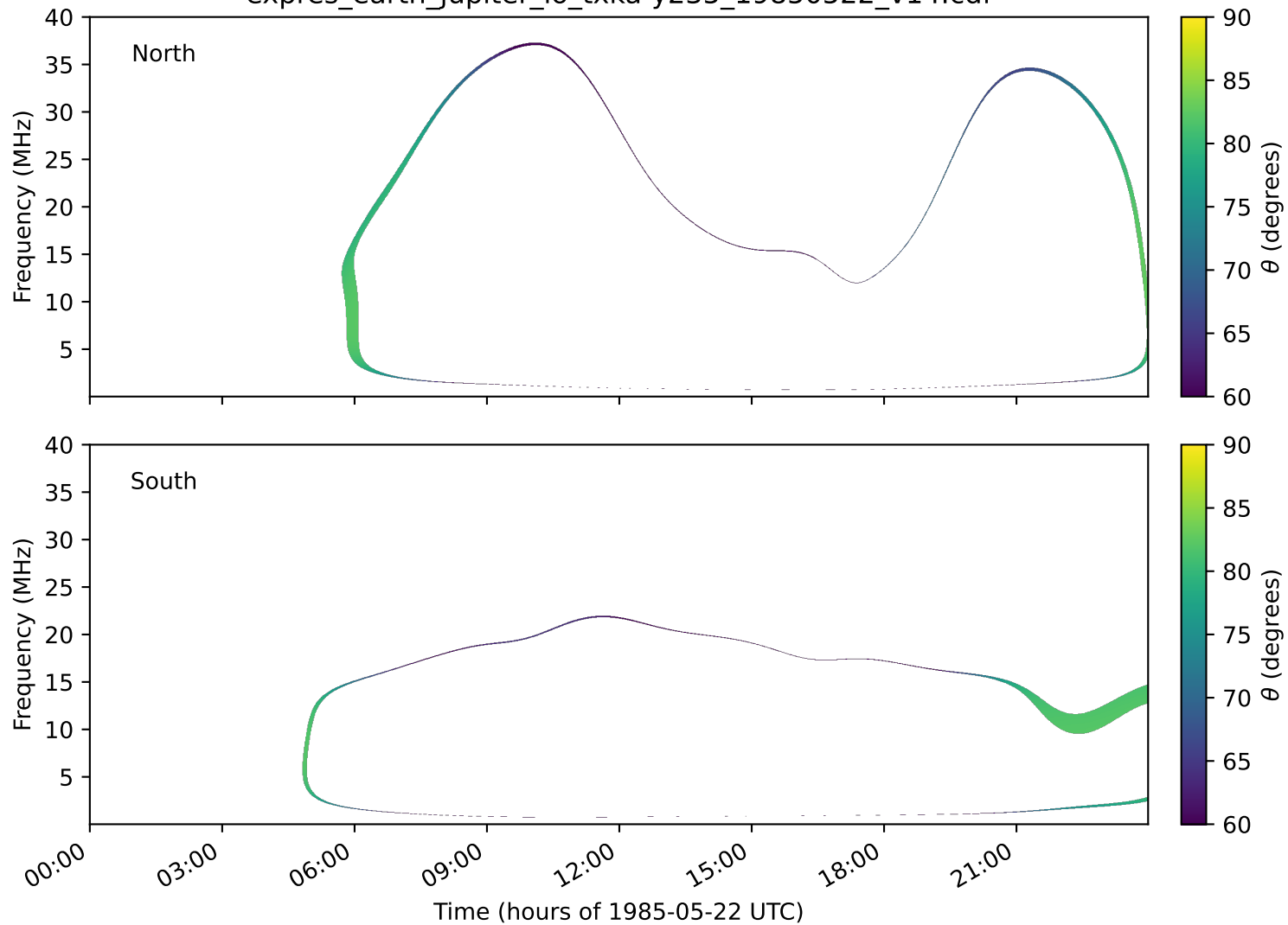
expres_earth_jupiter_io_txka-y235_19850522_v14.cdf
