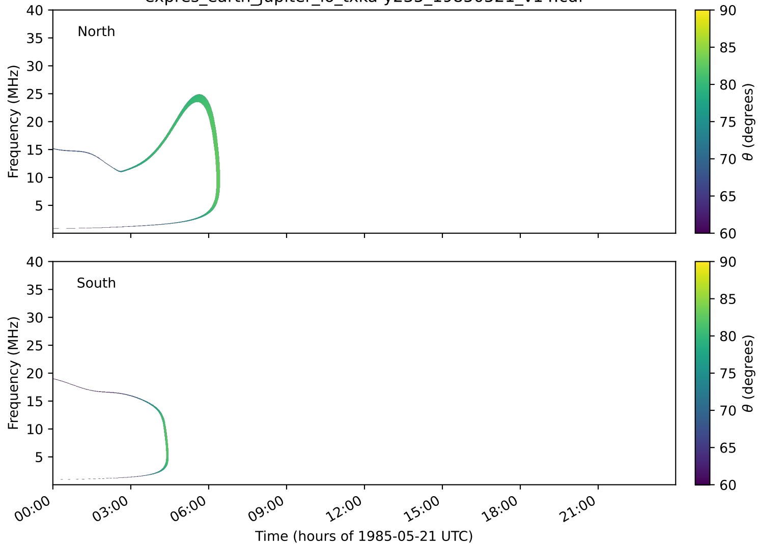
expres_earth_jupiter_io_txka-y235_19850521_v14.cdf
