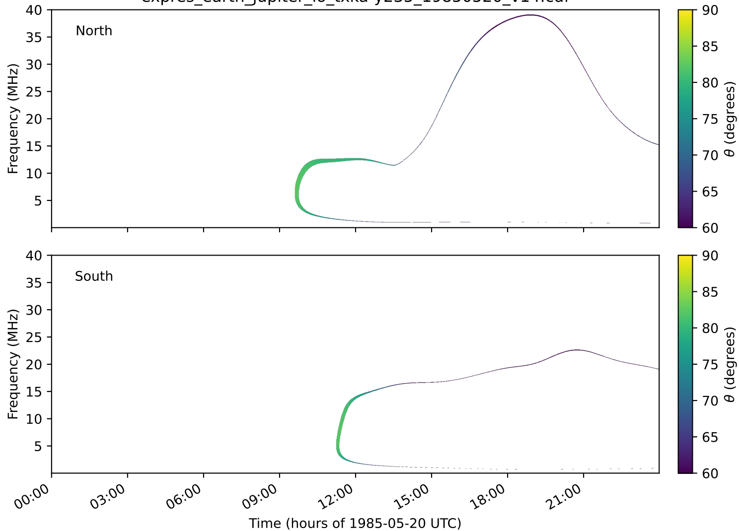
expres_earth_jupiter_io_txka-y235_19850520_v14.cdf
