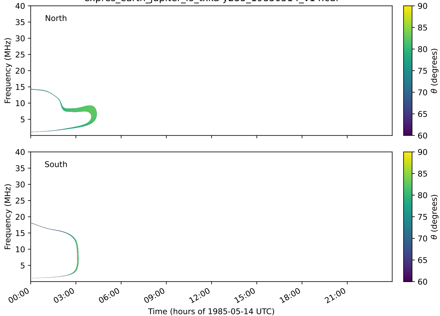
expres_earth_jupiter_io_txka-y235_19850514_v14.cdf
