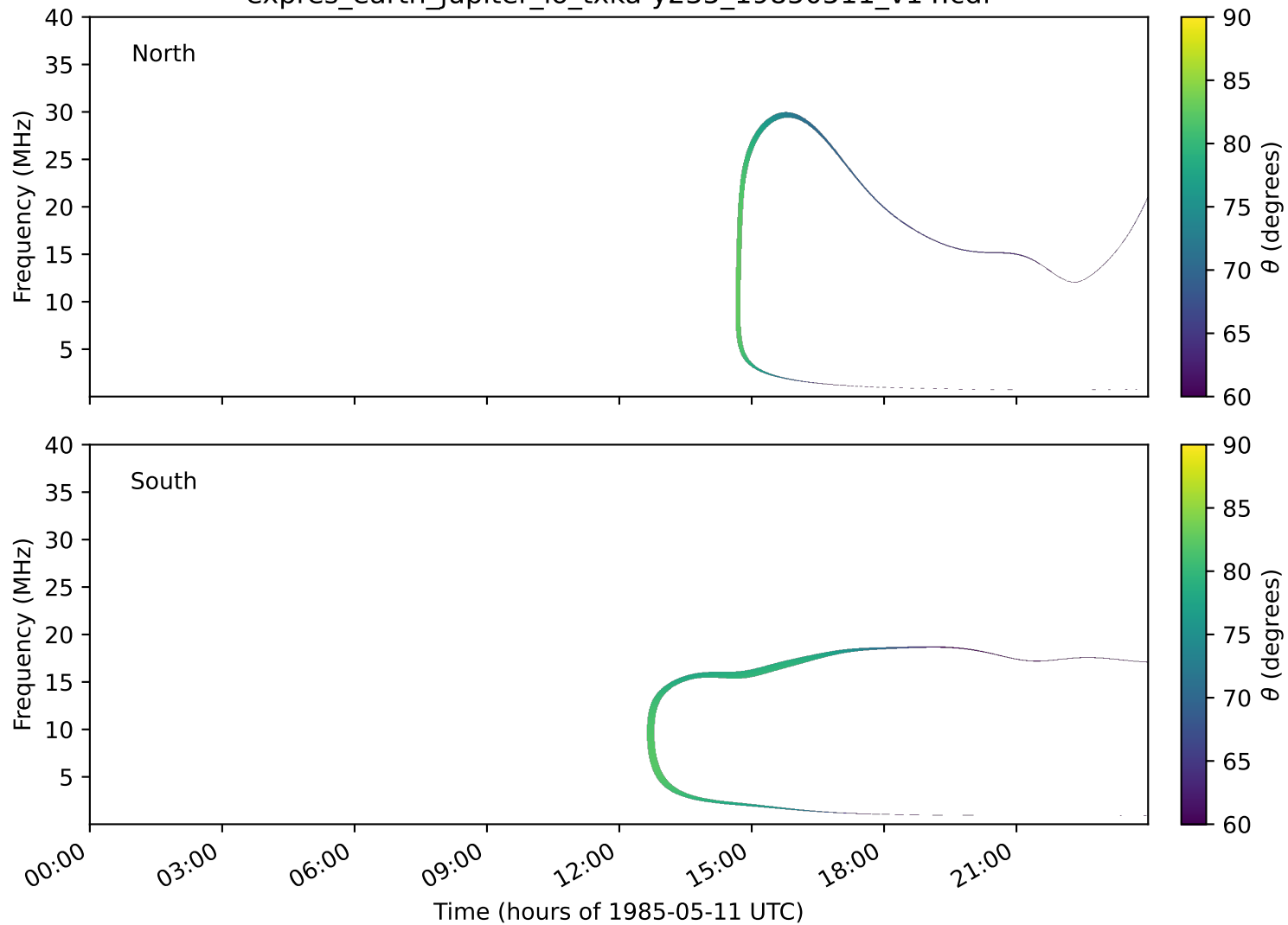
expres_earth_jupiter_io_txka-y235_19850511_v14.cdf
