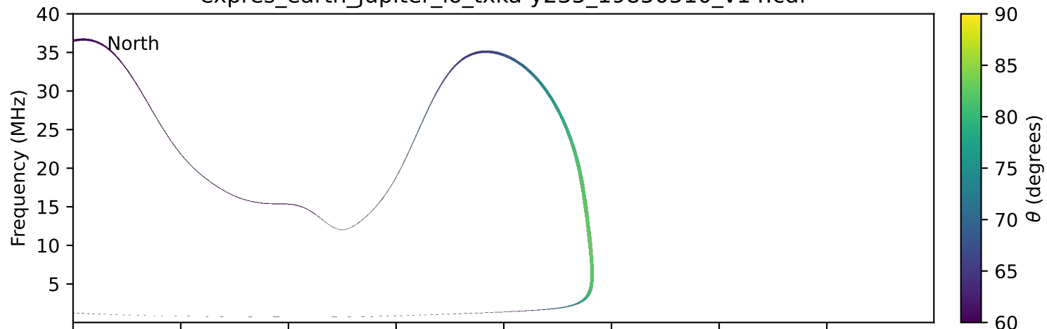
expres_earth_jupiter_io_txka-y235_19850510_v14.cdf
