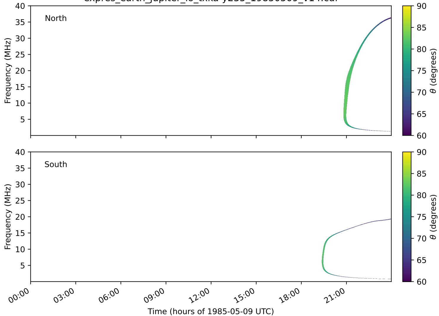
expres_earth_jupiter_io_txka-y235_19850509_v14.cdf
