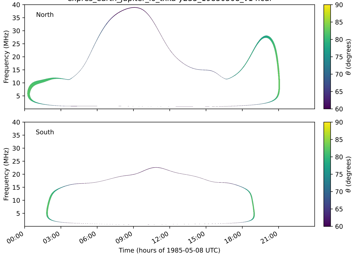
expres_earth_jupiter_io_txka-y235_19850508_v14.cdf
