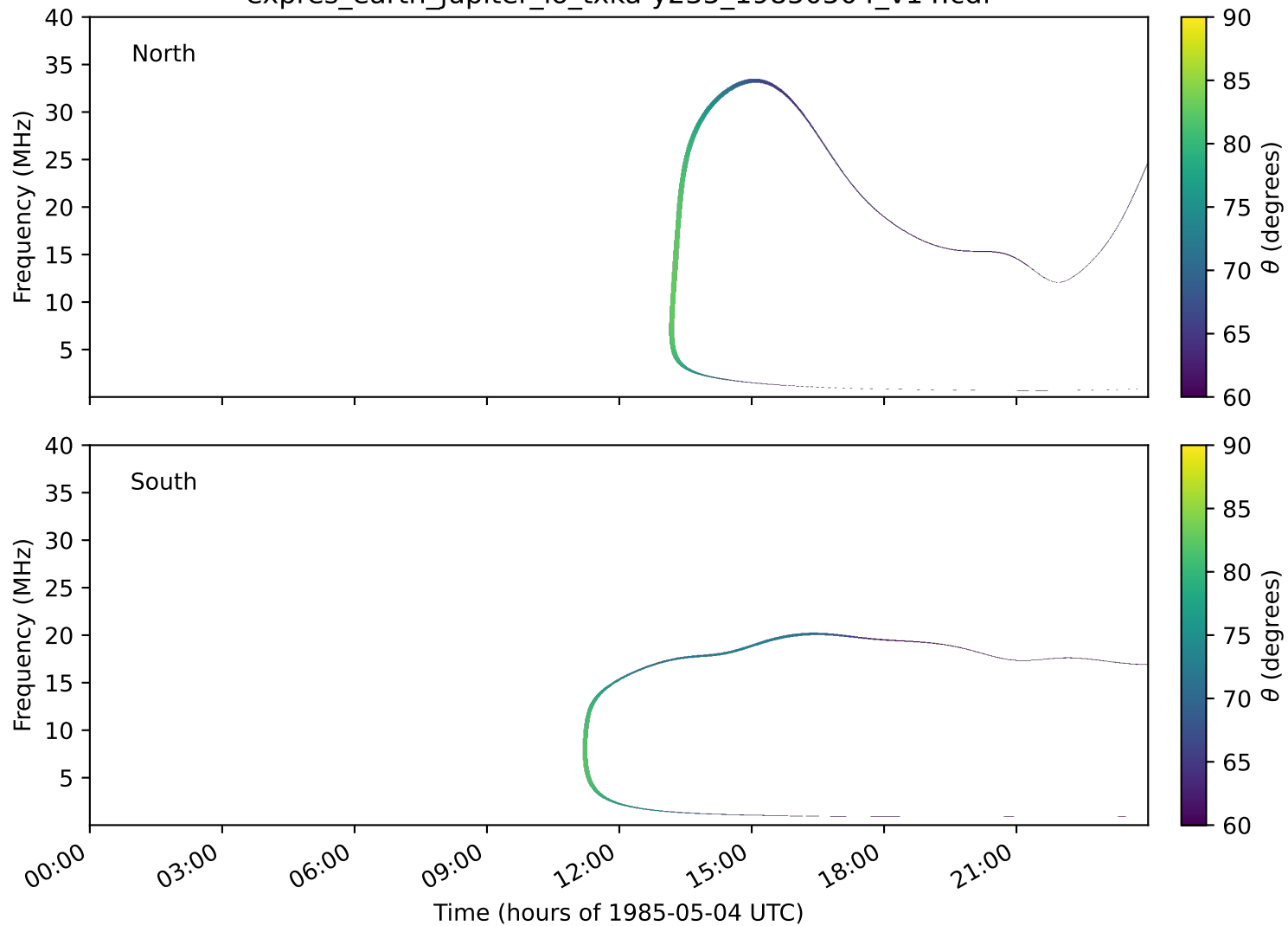
expres_earth_jupiter_io_txka-y235_19850504_v14.cdf
