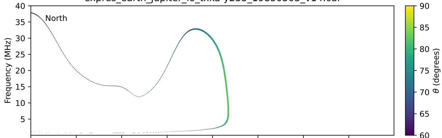
expres_earth_jupiter_io_txka-y235_19850503_v14.cdf
