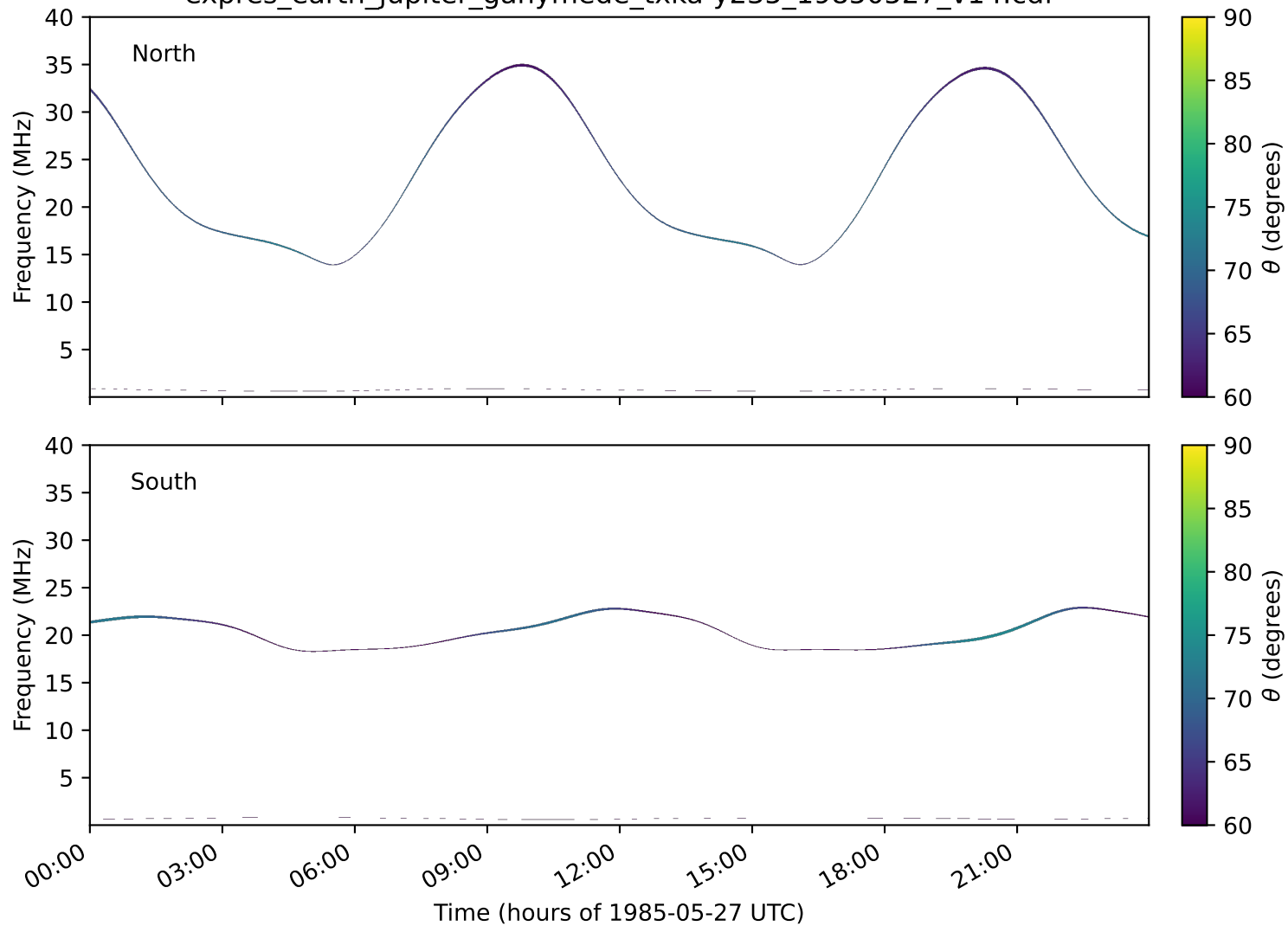
expres_earth_jupiter_ganymede_txka-y235_19850527_v14.cdf
