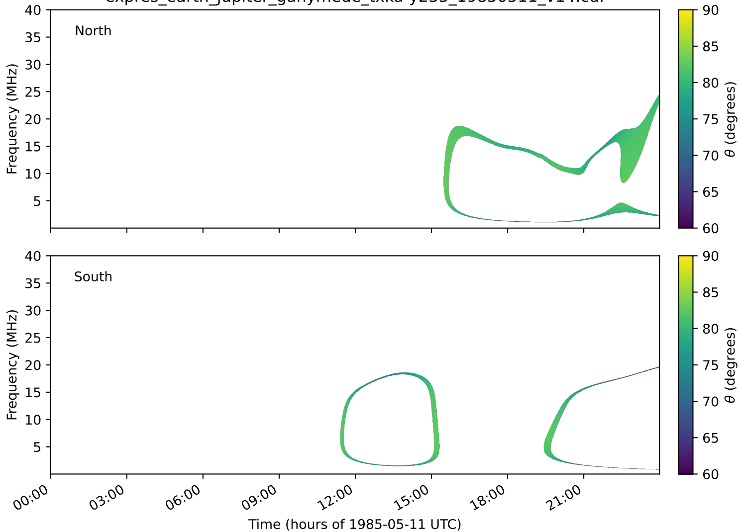
expres_earth_jupiter_ganymede_txka-y235_19850511_v14.cdf
