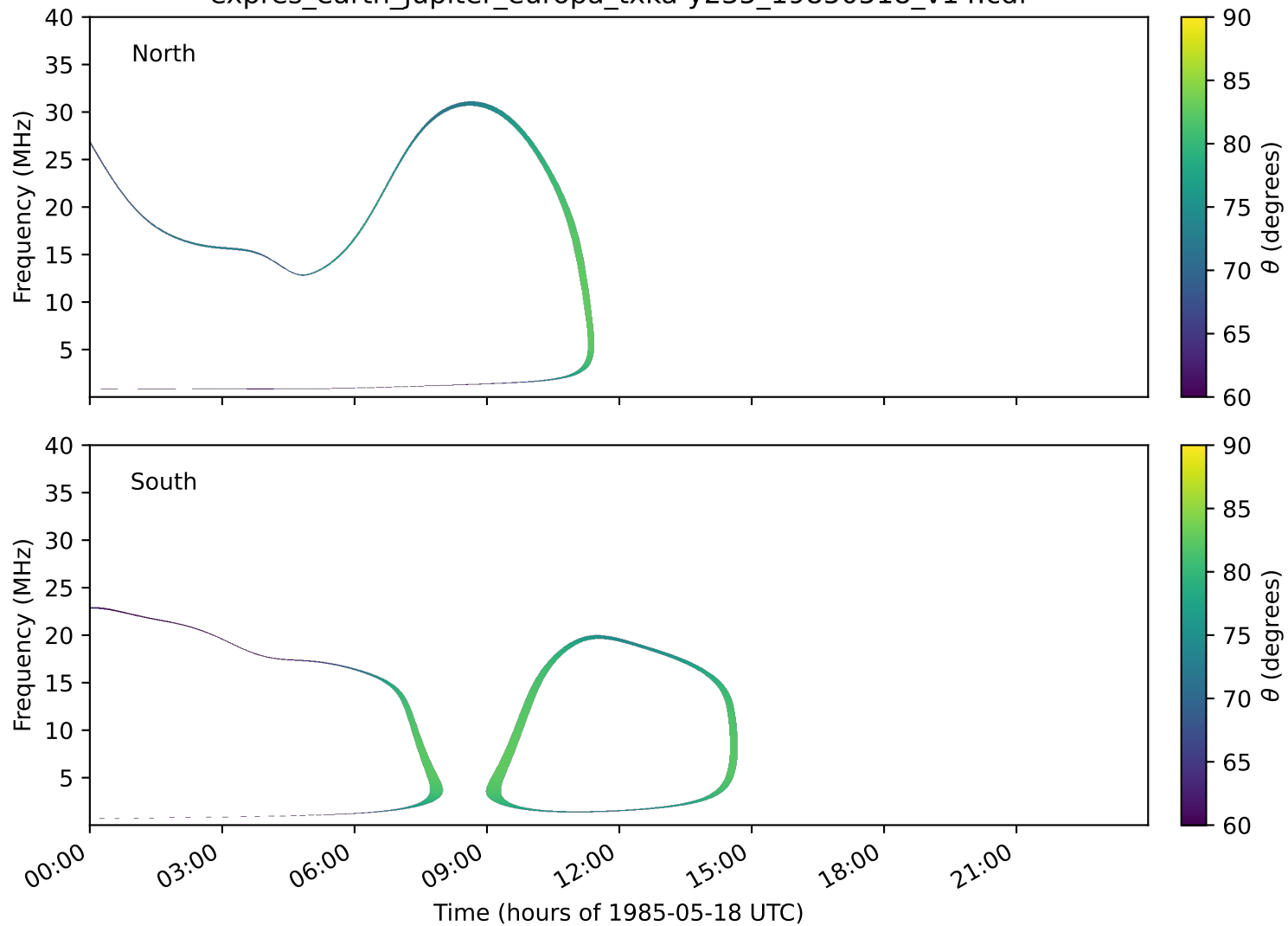
expres_earth_jupiter_europa_txka-y235_19850518_v14.cdf
