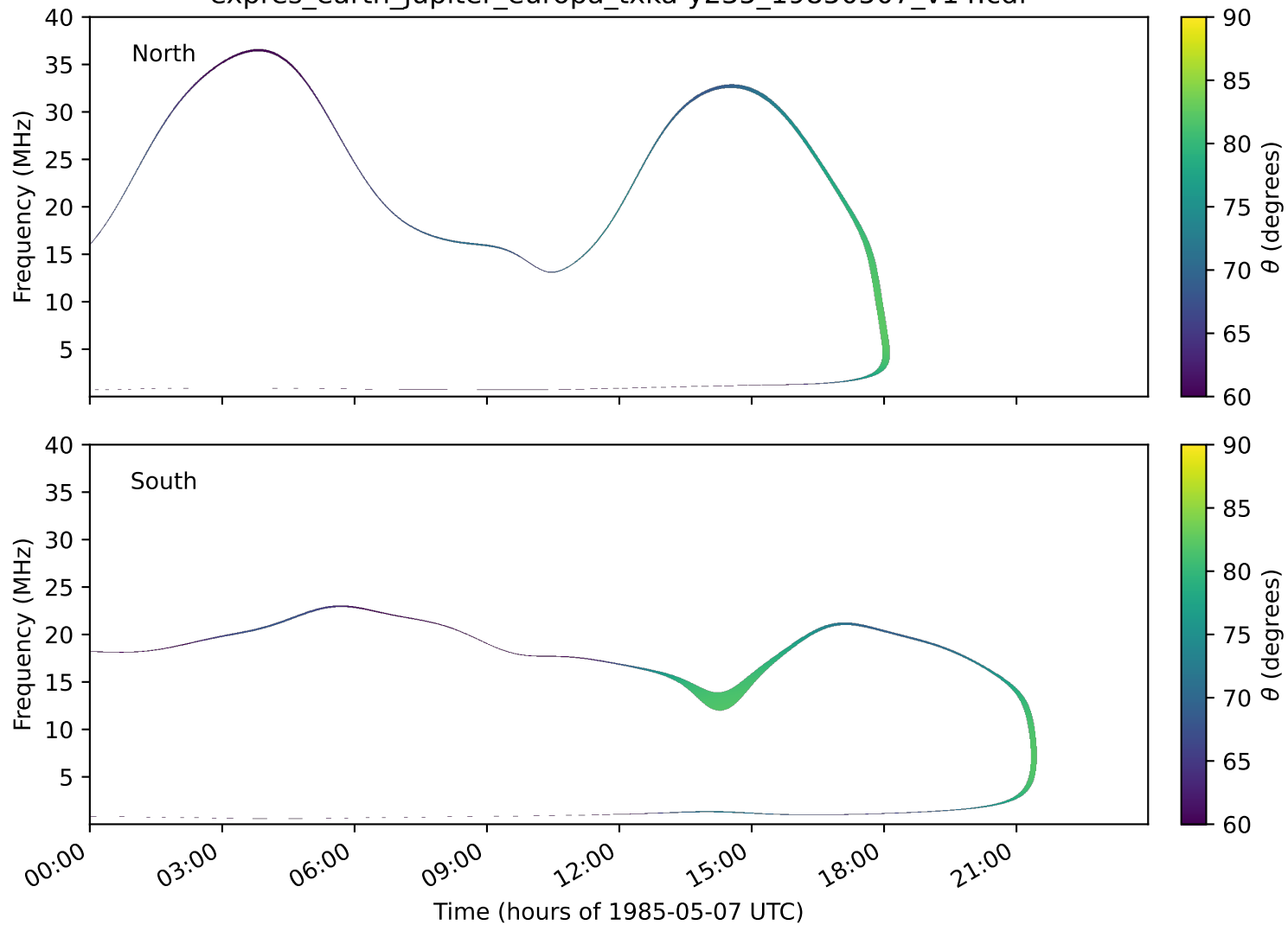
expres_earth_jupiter_europa_txka-y235_19850507_v14.cdf
