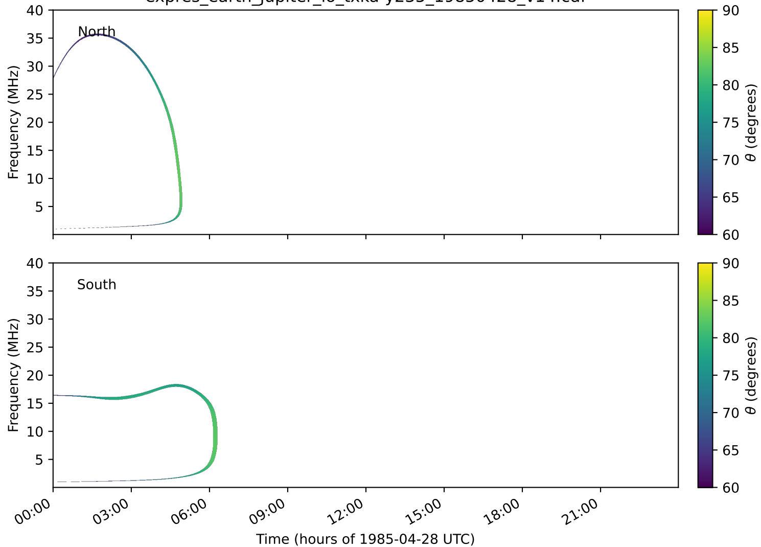
expres_earth_jupiter_io_txka-y235_19850428_v14.cdf
