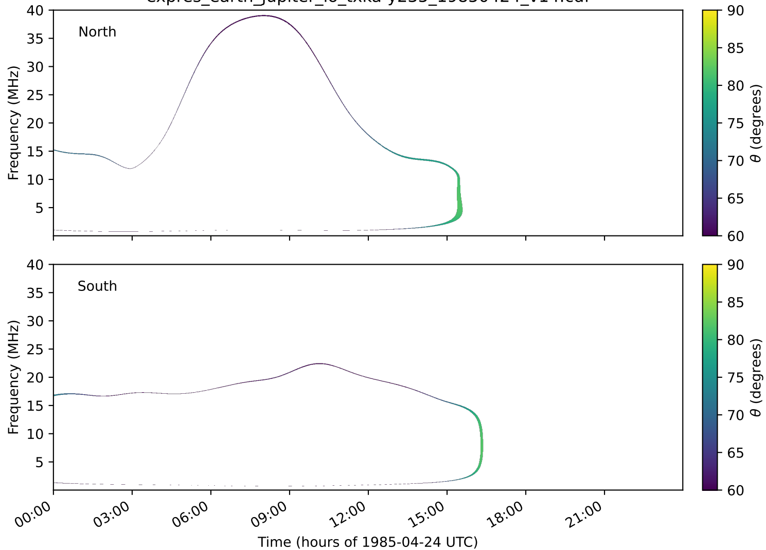
expres_earth_jupiter_io_txka-y235_19850424_v14.cdf
