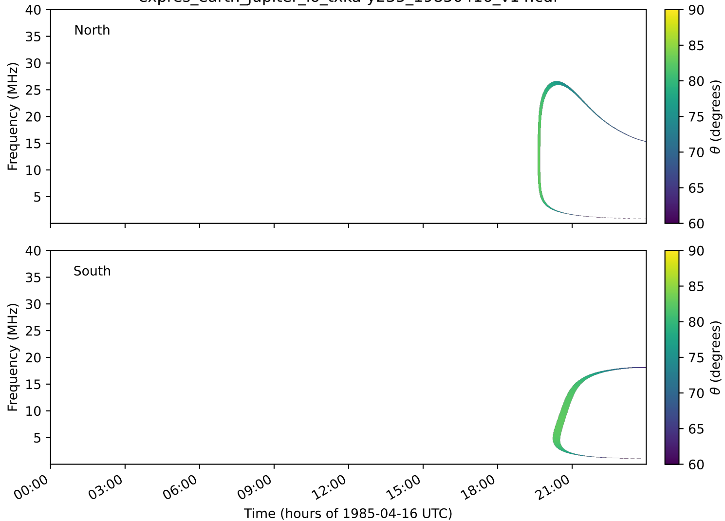
expres_earth_jupiter_io_txka-y235_19850416_v14.cdf
