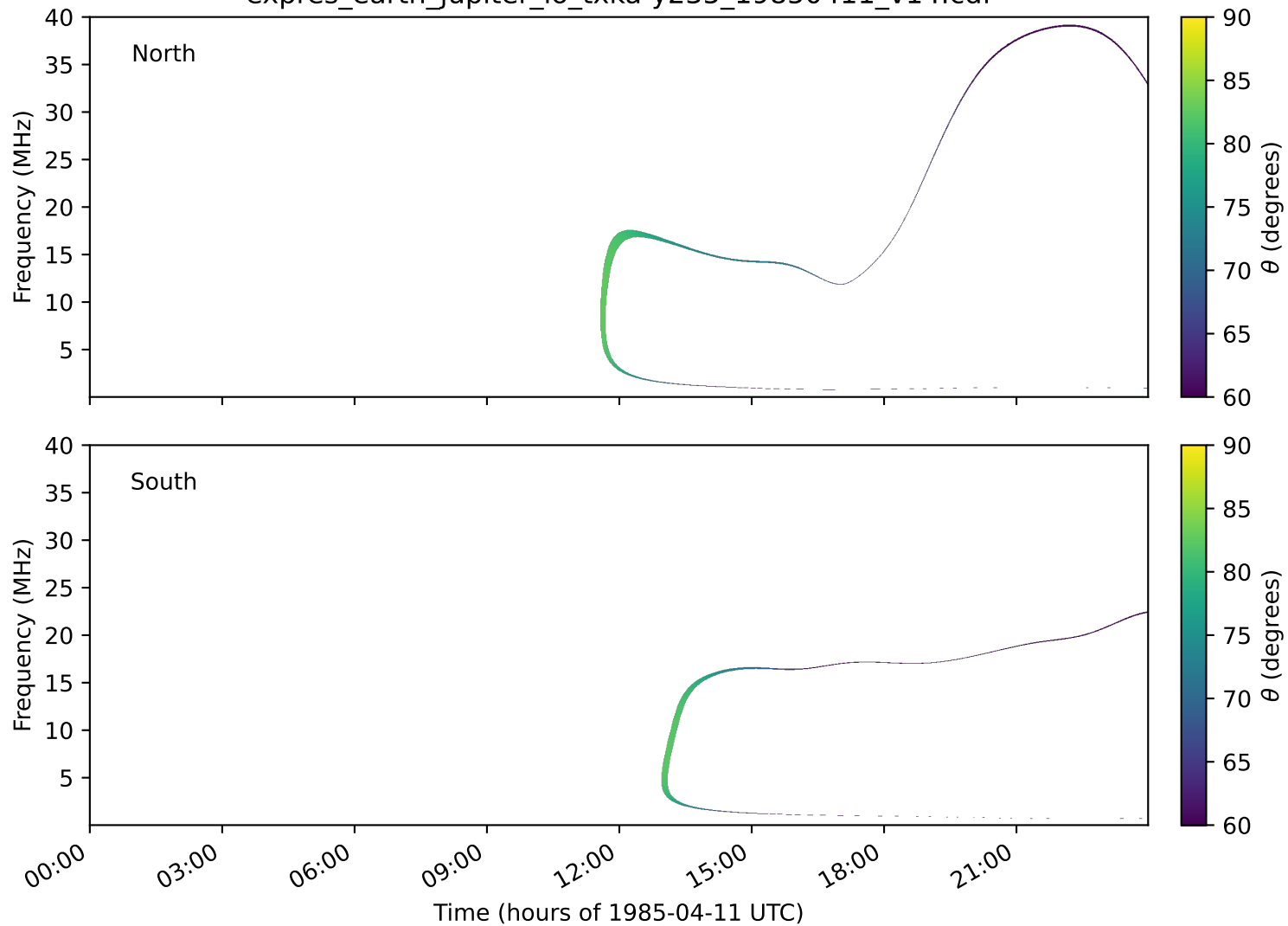
expres_earth_jupiter_io_txka-y235_19850411_v14.cdf
