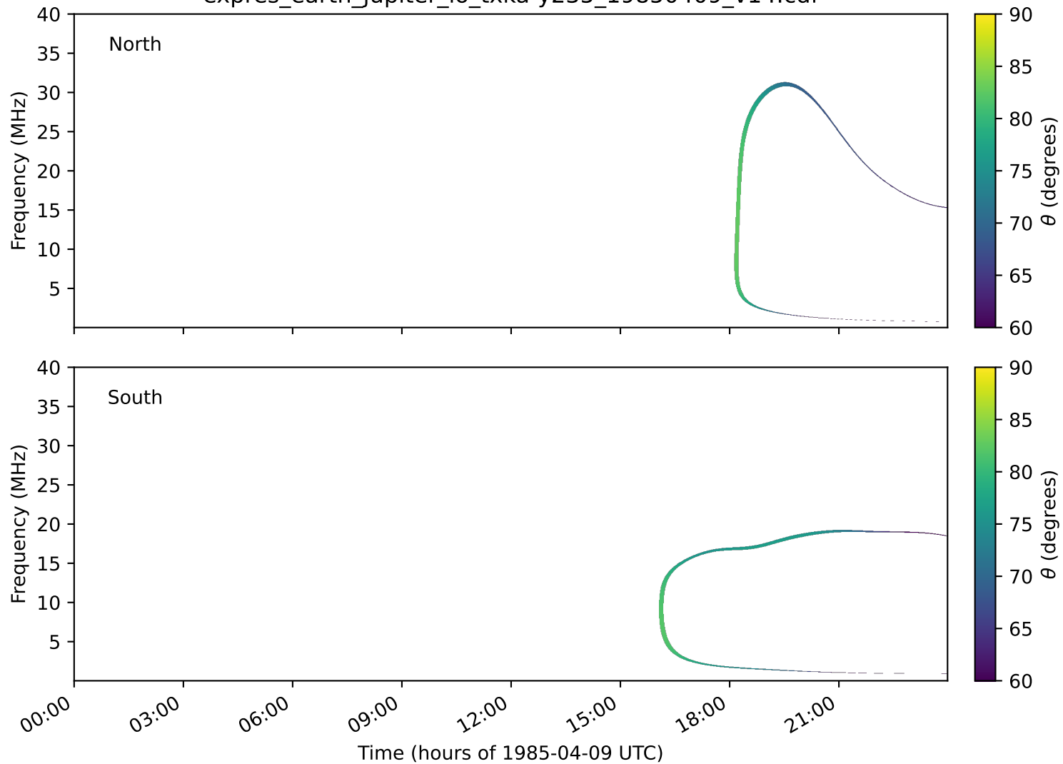
expres_earth_jupiter_io_txka-y235_19850409_v14.cdf
