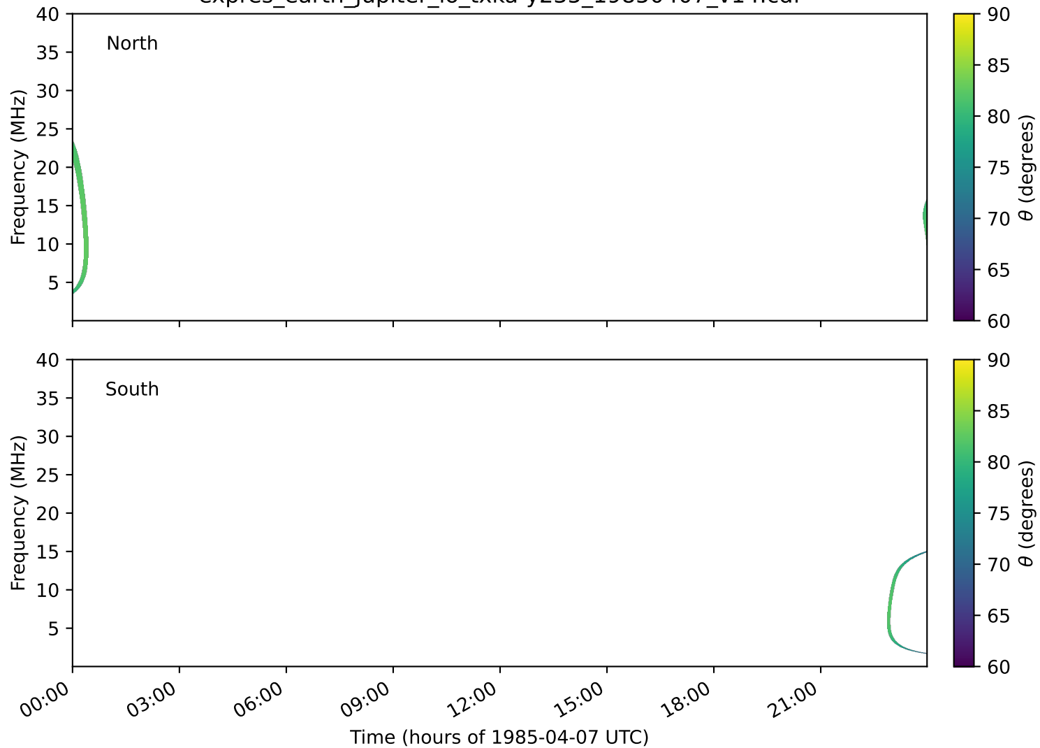
expres_earth_jupiter_io_txka-y235_19850407_v14.cdf
