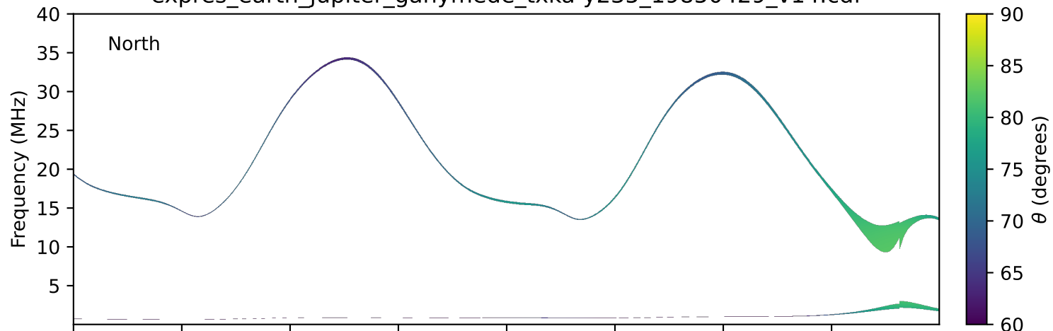
expres_earth_jupiter_ganymede_txka-y235_19850429_v14.cdf
