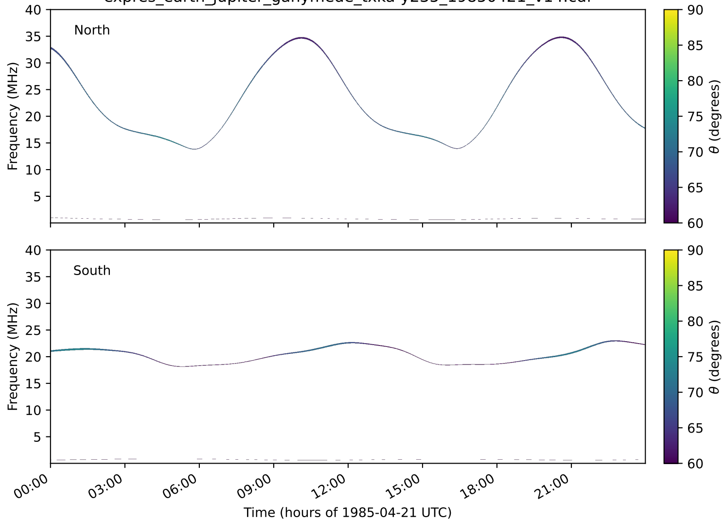
expres_earth_jupiter_ganymede_txka-y235_19850421_v14.cdf
